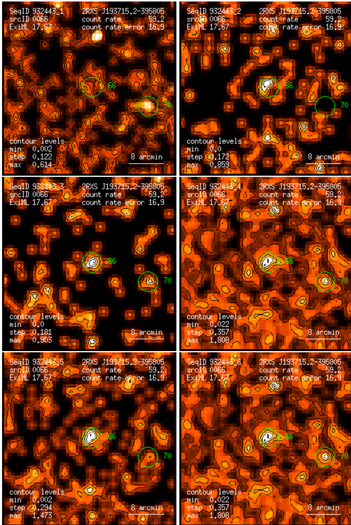
Figure 66: RASS 932443: detection 0066: band rate images, Gaussian filter: (1) PSPC channels 11 – 41, (2) 52 – 90, (3) 91 – 201, (4) 11 – 235, (5) 52 – 201, (6) 11 – 201. Broad band rates in counts/ks. Band rate contour levels in counts/ks/arcmin 2 .
