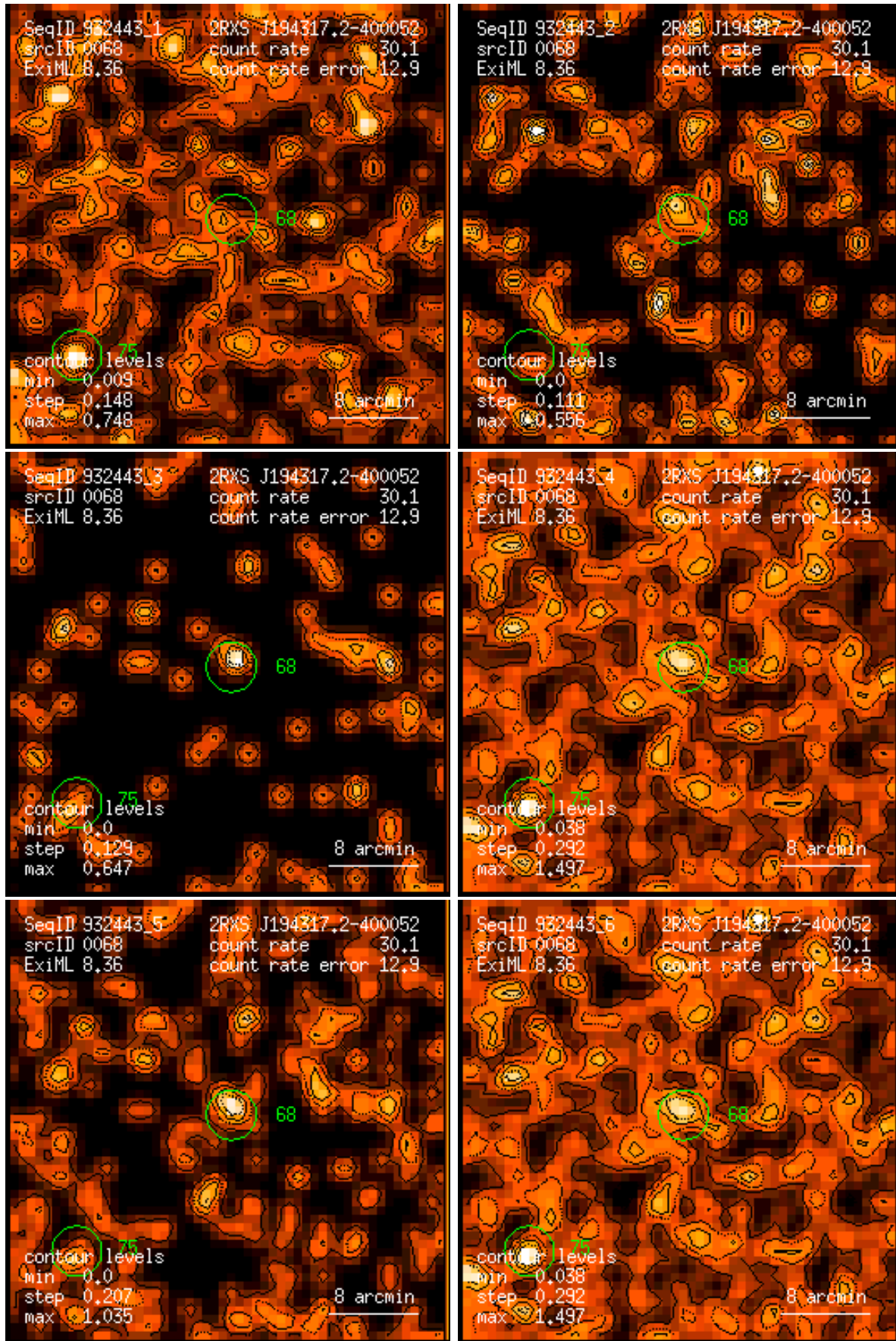
Figure 68: RASS 932443: detection 0068: band rate images, Gaussian filter: (1) PSPC channels 11 – 41, (2) 52 – 90, (3) 91 – 201, (4) 11 – 235, (5) 52 – 201, (6) 11 – 201. Broad band rates in counts/ks. Band rate contour levels in counts/ks/arcmin 2 .
