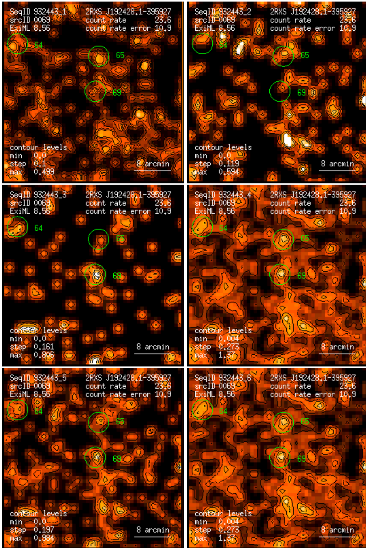
Figure 69: RASS 932443: detection 0069: band rate images, Gaussian filter: (1) PSPC channels 11 – 41, (2) 52 – 90, (3) 91 – 201, (4) 11 – 235, (5) 52 – 201, (6) 11 – 201. Broad band rates in counts/ks. Band rate contour levels in counts/ks/arcmin 2 .
