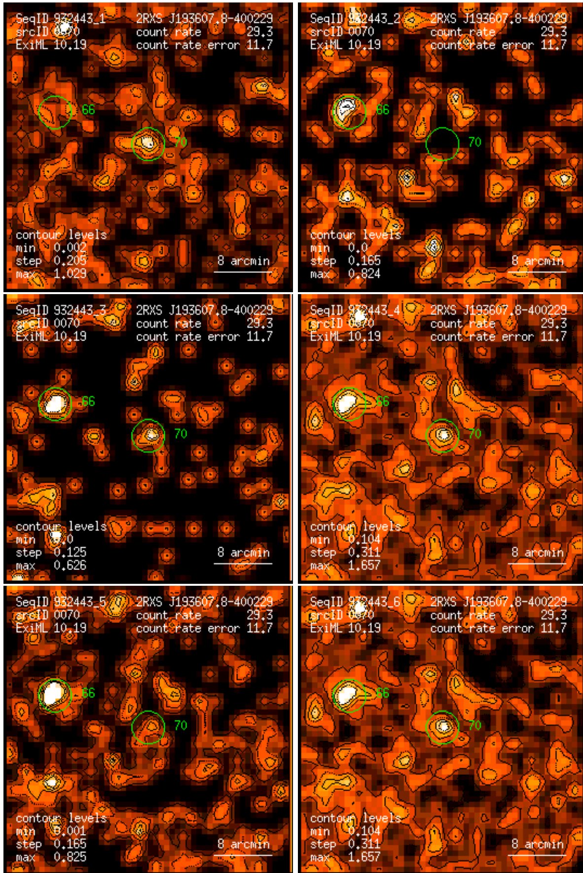
Figure 70: RASS 932443: detection 0070: band rate images, Gaussian filter: (1) PSPC channels 11 – 41, (2) 52 – 90, (3) 91 – 201, (4) 11 – 235, (5) 52 – 201, (6) 11 – 201. Broad band rates in counts/ks. Band rate contour levels in counts/ks/arcmin 2 .
