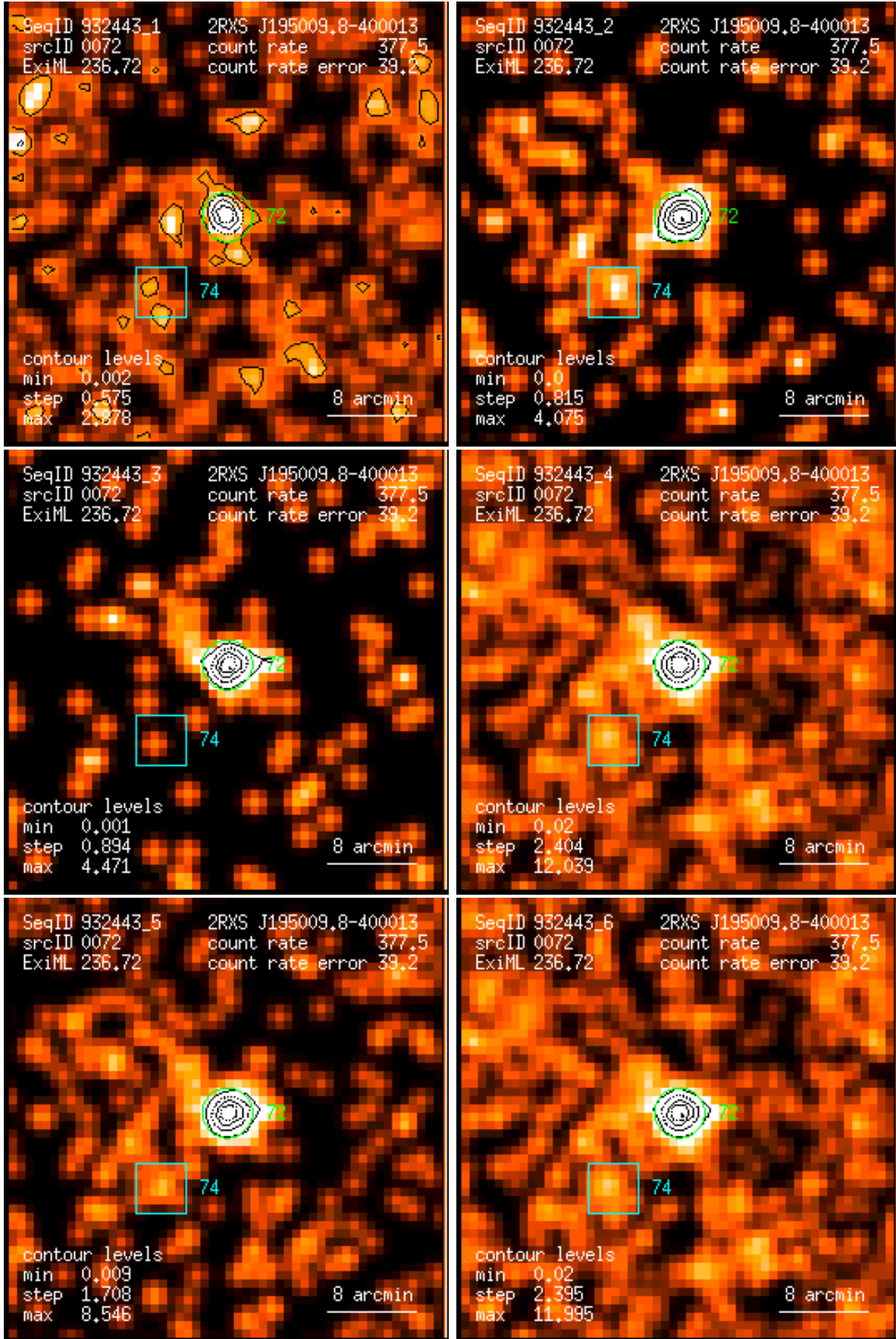
Figure 72: RASS 932443: detection 0072: band rate images, Gaussian filter: (1) PSPC channels 11 – 41, (2) 52 – 90, (3) 91 – 201, (4) 11 – 235, (5) 52 – 201, (6) 11 – 201. Broad band rates in counts/ks. Band rate contour levels in counts/ks/arcmin 2 .
