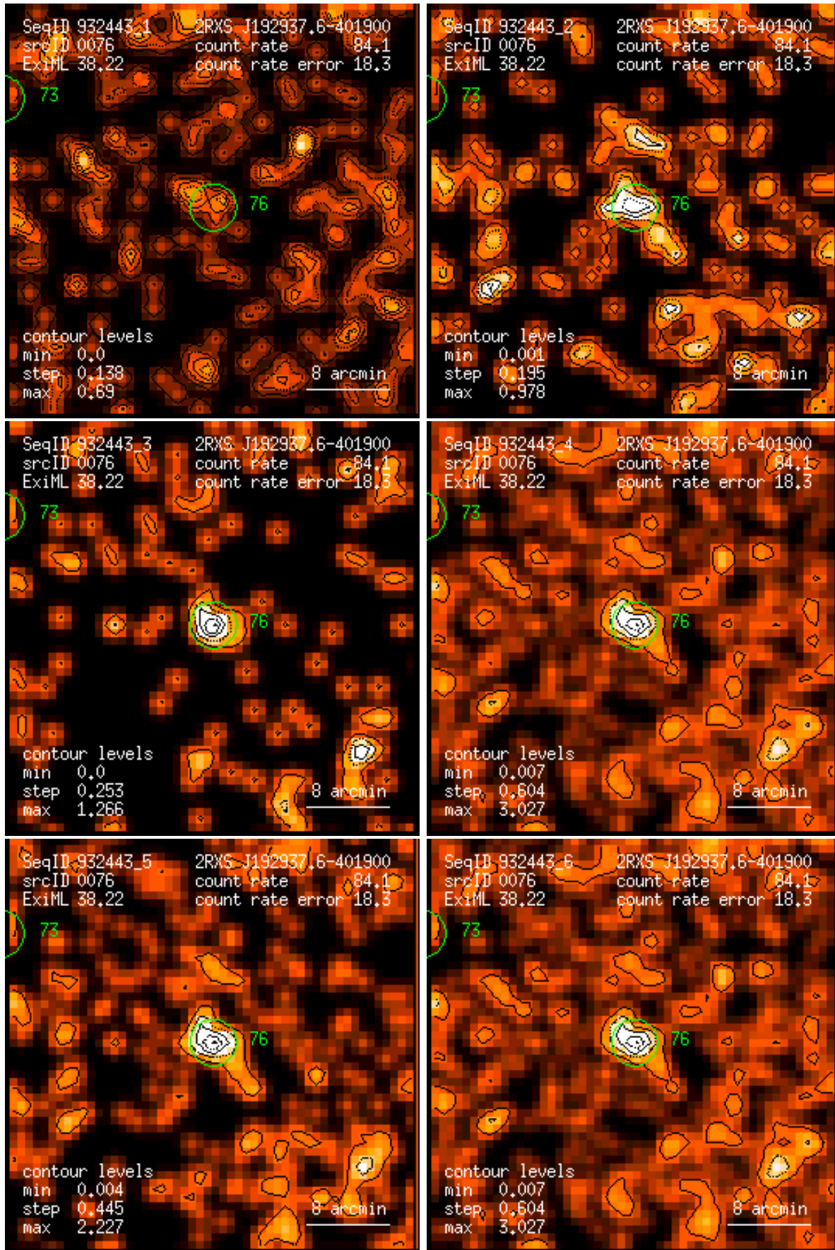
Figure 76: RASS 932443: detection 0076: band rate images, Gaussian filter: (1) PSPC channels 11 – 41, (2) 52 – 90, (3) 91 – 201, (4) 11 – 235, (5) 52 – 201, (6) 11 – 201. Broad band rates in counts/ks. Band rate contour levels in counts/ks/arcmin 2 .
