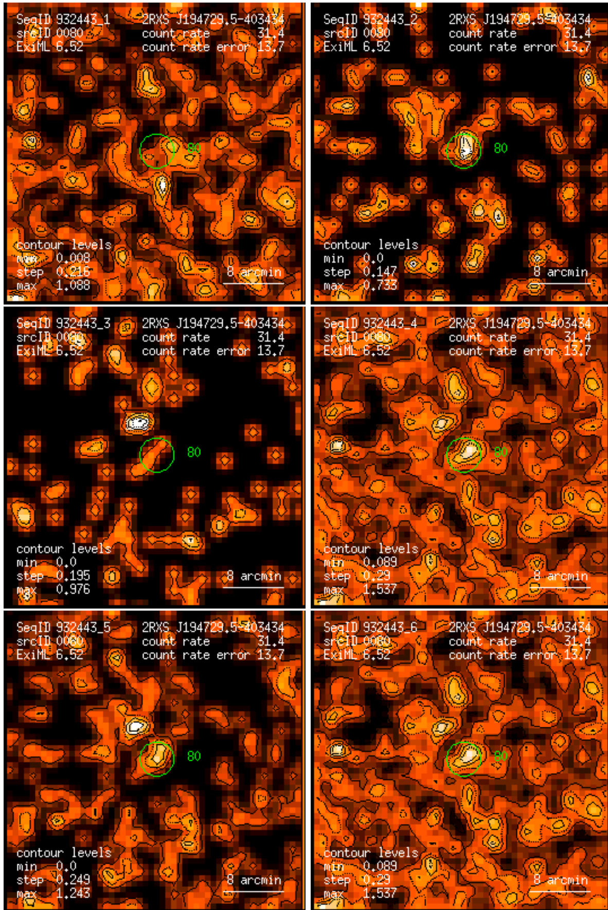
Figure 80: RASS 932443: detection 0080: band rate images, Gaussian filter: (1) PSPC channels 11 – 41, (2) 52 – 90, (3) 91 – 201, (4) 11 – 235, (5) 52 – 201, (6) 11 – 201. Broad band rates in counts/ks. Band rate contour levels in counts/ks/arcmin 2 .
