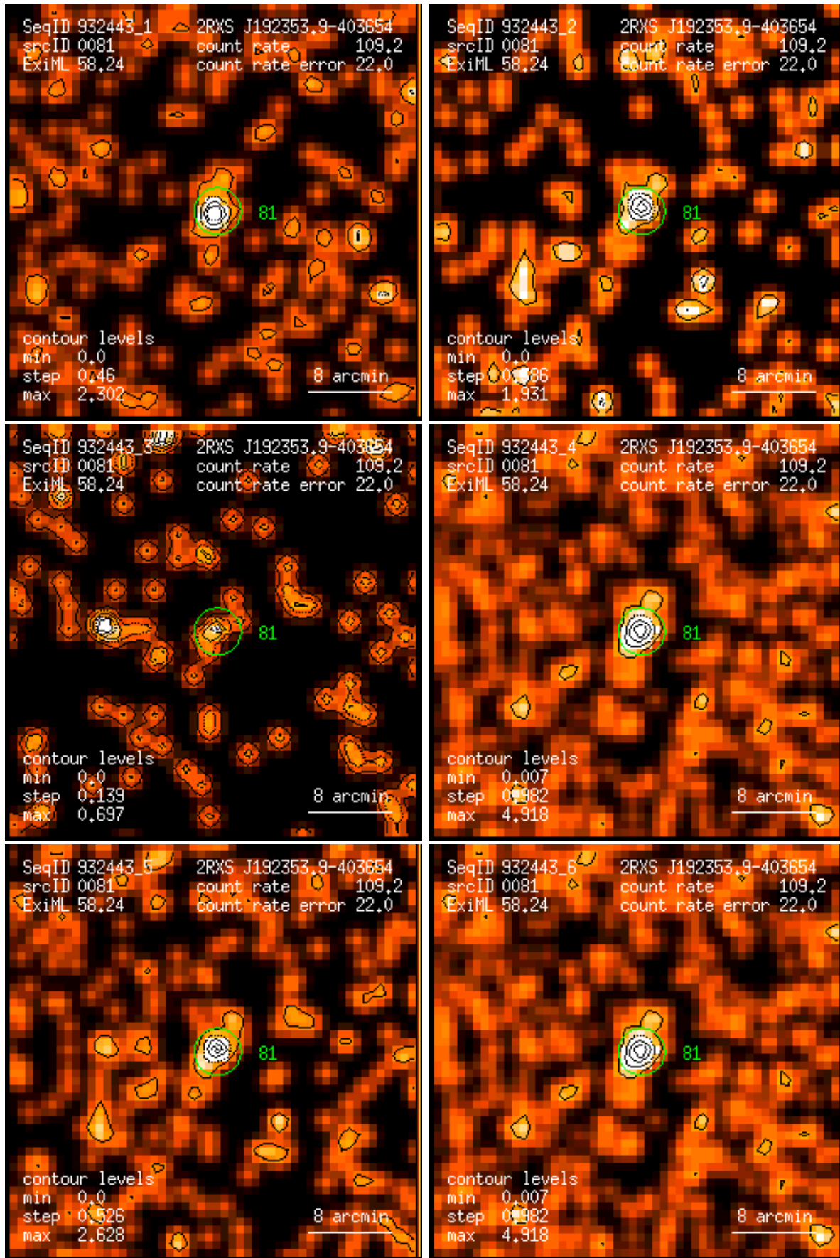
Figure 81: RASS 932443: detection 0081: band rate images, Gaussian filter: (1) PSPC channels 11 – 41, (2) 52 – 90, (3) 91 – 201, (4) 11 – 235, (5) 52 – 201, (6) 11 – 201. Broad band rates in counts/ks. Band rate contour levels in counts/ks/arcmin 2 .
