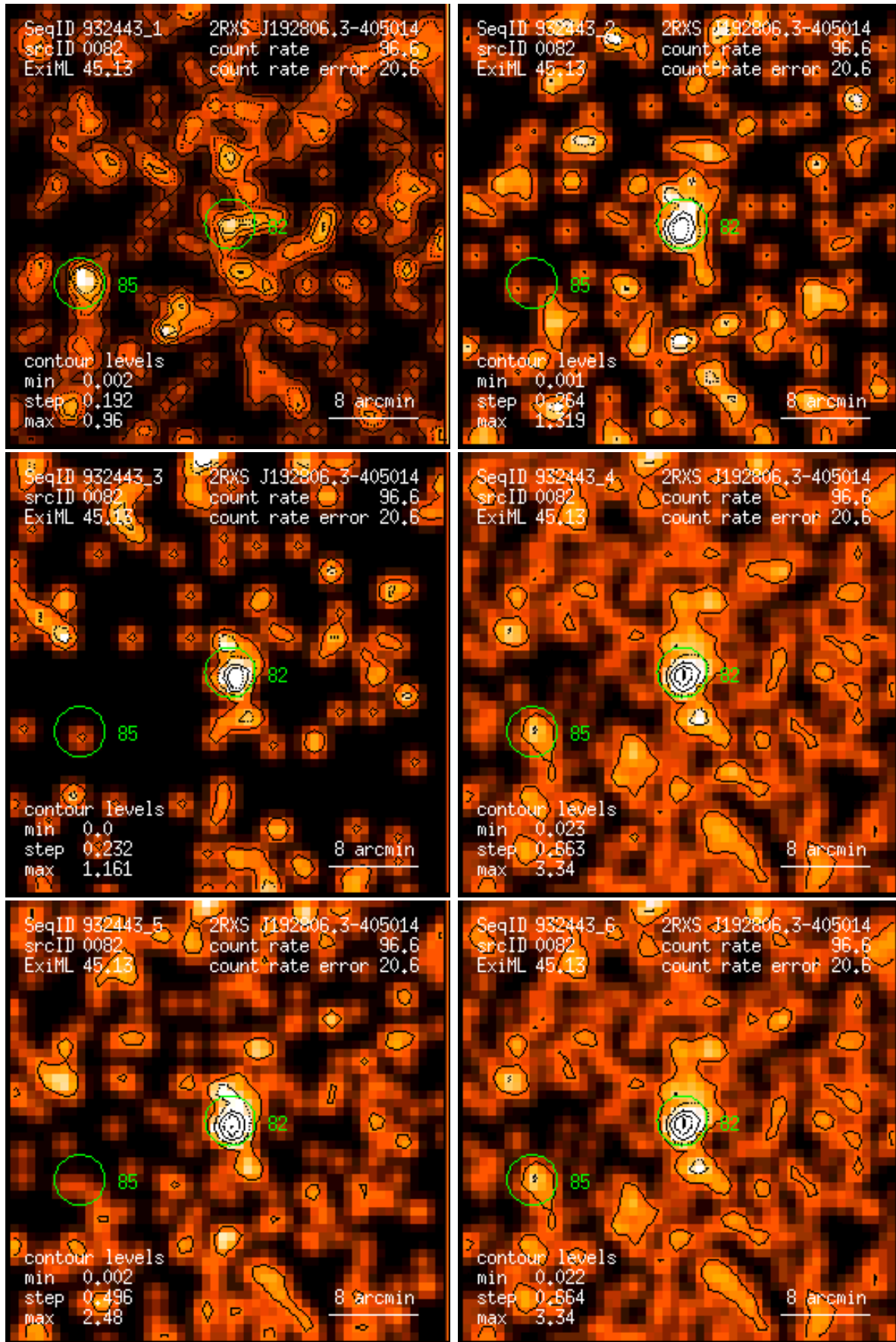
Figure 82: RASS 932443: detection 0082: band rate images, Gaussian filter: (1) PSPC channels 11 – 41, (2) 52 – 90, (3) 91 – 201, (4) 11 – 235, (5) 52 – 201, (6) 11 – 201. Broad band rates in counts/ks. Band rate contour levels in counts/ks/arcmin 2 .
