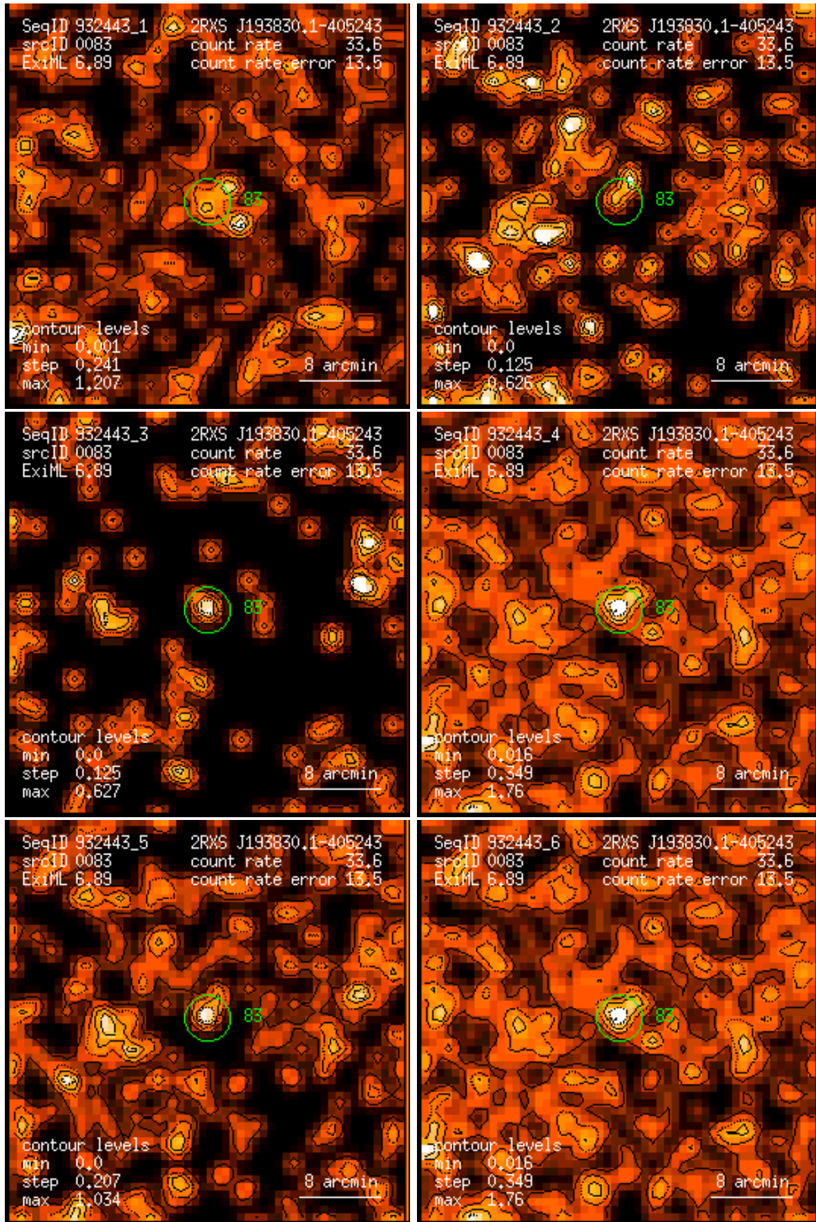
Figure 83: RASS 932443: detection 0083: band rate images, Gaussian filter: (1) PSPC channels 11 – 41, (2) 52 – 90, (3) 91 – 201, (4) 11 – 235, (5) 52 – 201, (6) 11 – 201. Broad band rates in counts/ks. Band rate contour levels in counts/ks/arcmin 2 .
