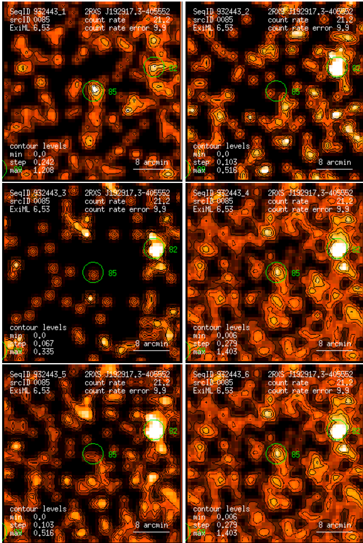
Figure 85: RASS 932443: detection 0085: band rate images, Gaussian filter: (1) PSPC channels 11 – 41, (2) 52 – 90, (3) 91 – 201, (4) 11 – 235, (5) 52 – 201, (6) 11 – 201. Broad band rates in counts/ks. Band rate contour levels in counts/ks/arcmin 2 .
