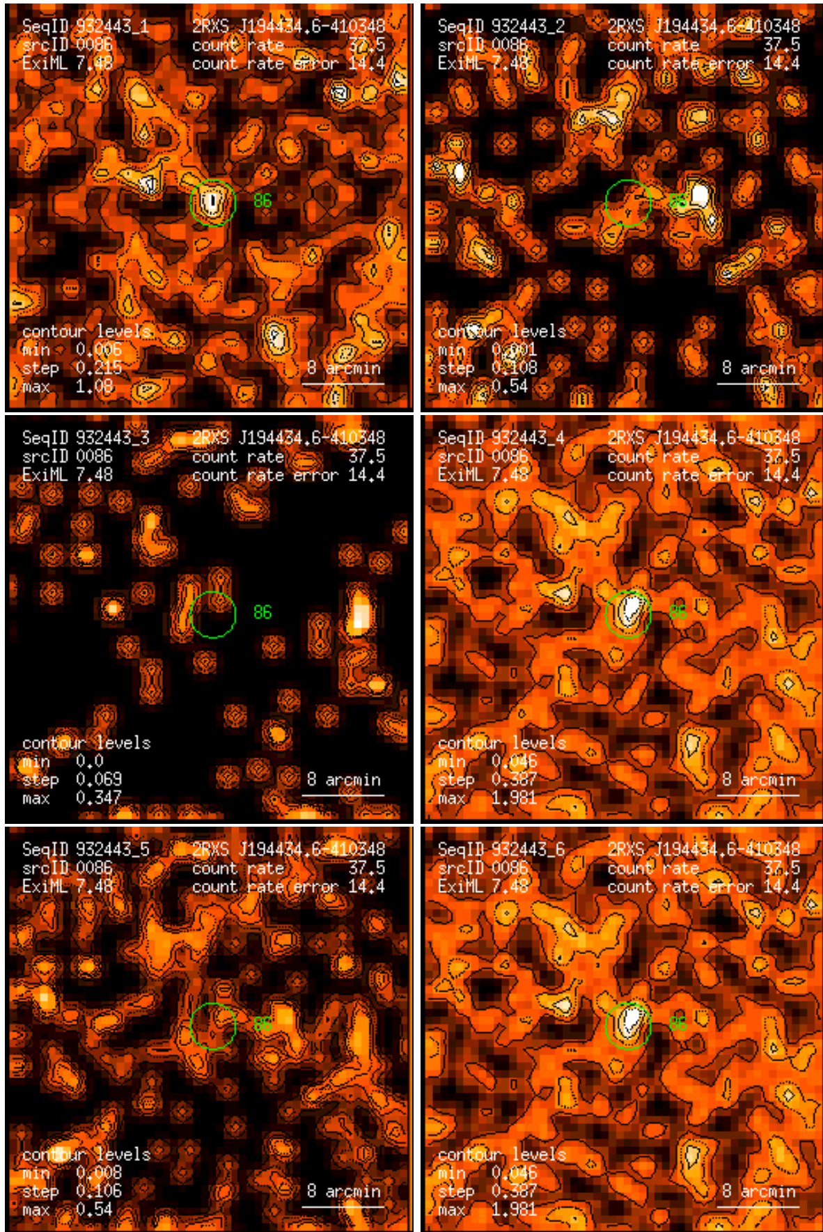
Figure 86: RASS 932443: detection 0086: band rate images, Gaussian filter: (1) PSPC channels 11 – 41, (2) 52 – 90, (3) 91 – 201, (4) 11 – 235, (5) 52 – 201, (6) 11 – 201. Broad band rates in counts/ks. Band rate contour levels in counts/ks/arcmin 2 .
