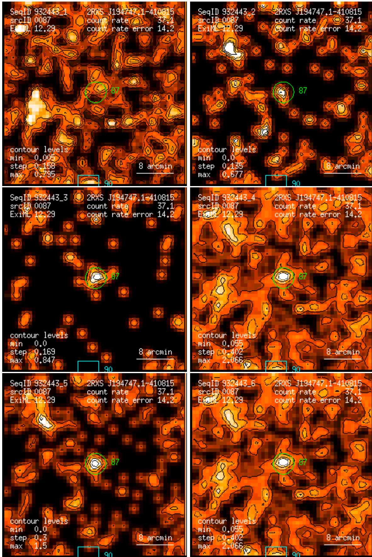
Figure 87: RASS 932443: detection 0087: band rate images, Gaussian filter: (1) PSPC channels 11 – 41, (2) 52 – 90, (3) 91 – 201, (4) 11 – 235, (5) 52 – 201, (6) 11 – 201. Broad band rates in counts/ks. Band rate contour levels in counts/ks/arcmin 2 .
