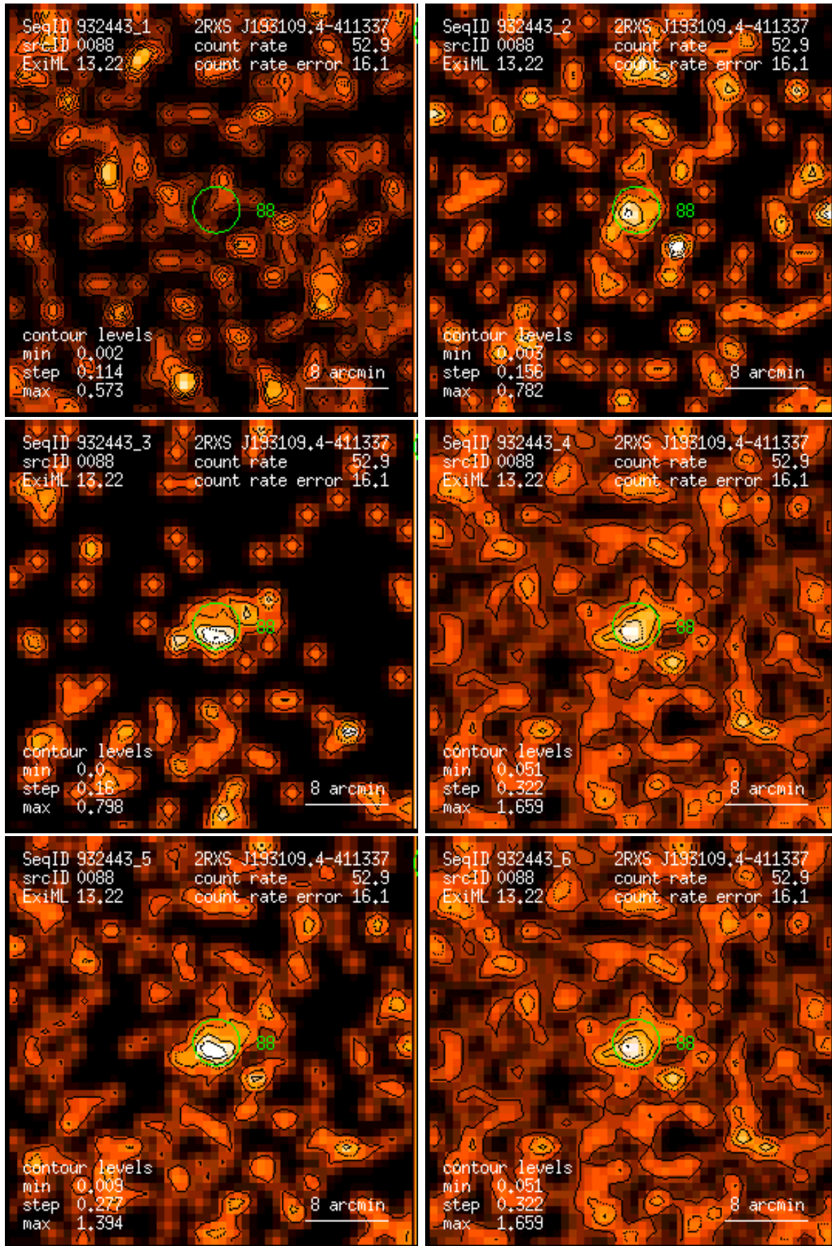
Figure 88: RASS 932443: detection 0088: band rate images, Gaussian filter: (1) PSPC channels 11 – 41, (2) 52 – 90, (3) 91 – 201, (4) 11 – 235, (5) 52 – 201, (6) 11 – 201. Broad band rates in counts/ks. Band rate contour levels in counts/ks/arcmin 2 .
