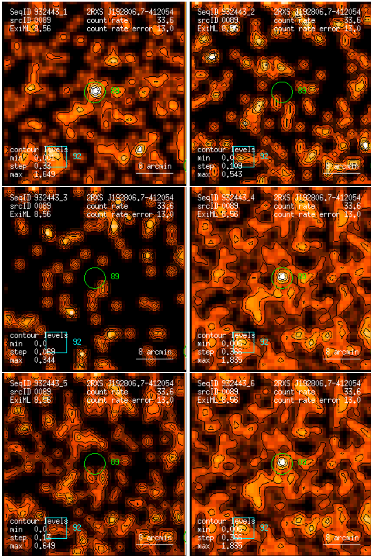
Figure 89: RASS 932443: detection 0089: band rate images, Gaussian filter: (1) PSPC channels 11 – 41, (2) 52 – 90, (3) 91 – 201, (4) 11 – 235, (5) 52 – 201, (6) 11 – 201. Broad band rates in counts/ks. Band rate contour levels in counts/ks/arcmin 2 .
