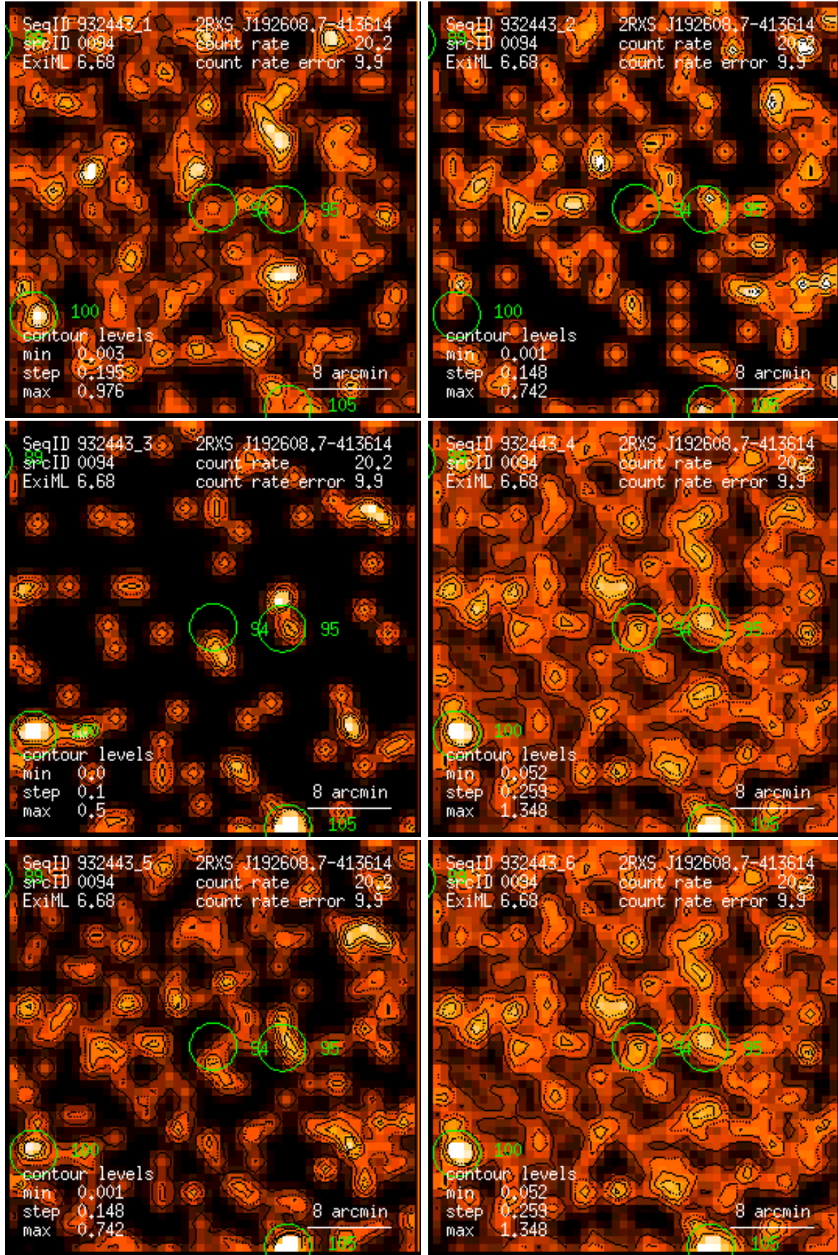
Figure 94: RASS 932443: detection 0094: band rate images, Gaussian filter: (1) PSPC channels 11 – 41, (2) 52 – 90, (3) 91 – 201, (4) 11 – 235, (5) 52 – 201, (6) 11 – 201. Broad band rates in counts/ks. Band rate contour levels in counts/ks/arcmin 2 .
