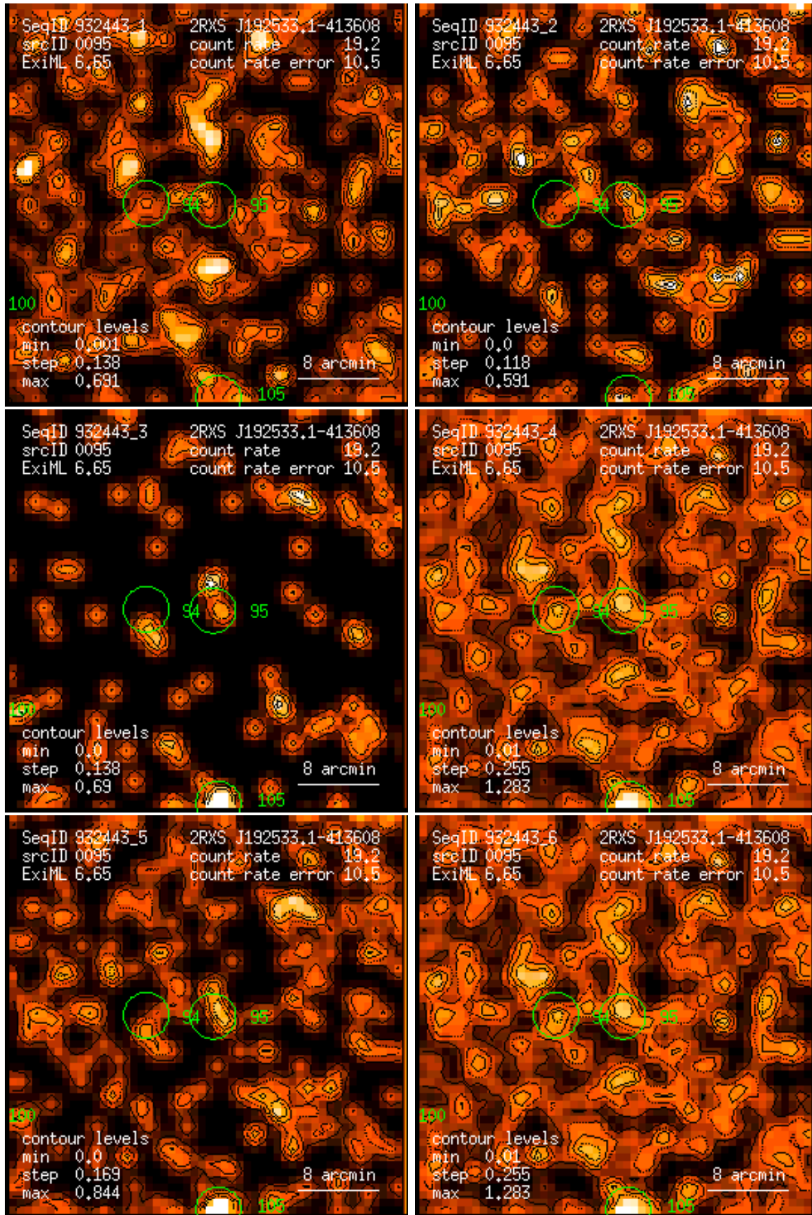
Figure 95: RASS 932443: detection 0095: band rate images, Gaussian filter: (1) PSPC channels 11 – 41, (2) 52 – 90, (3) 91 – 201, (4) 11 – 235, (5) 52 – 201, (6) 11 – 201. Broad band rates in counts/ks. Band rate contour levels in counts/ks/arcmin 2 .
