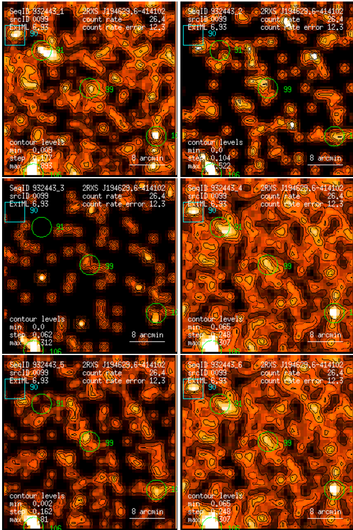
Figure 99: RASS 932443: detection 0099: band rate images, Gaussian filter: (1) PSPC channels 11 – 41, (2) 52 – 90, (3) 91 – 201, (4) 11 – 235, (5) 52 – 201, (6) 11 – 201. Broad band rates in counts/ks. Band rate contour levels in counts/ks/arcmin 2 .
