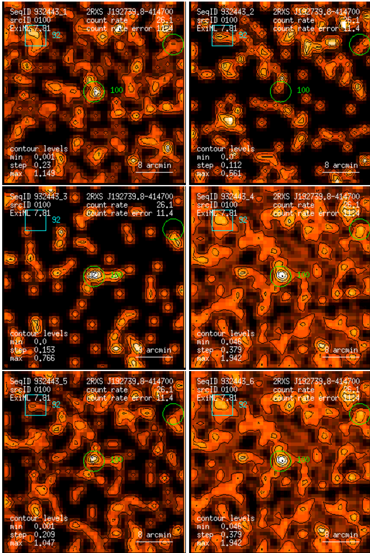
Figure 100: RASS 932443: detection 0100: band rate images, Gaussian filter: (1) PSPC channels 11 – 41, (2) 52 – 90, (3) 91 – 201, (4) 11 – 235, (5) 52 – 201, (6) 11 – 201. Broad band rates in counts/ks. Band rate contour levels in counts/ks/arcmin 2 .
