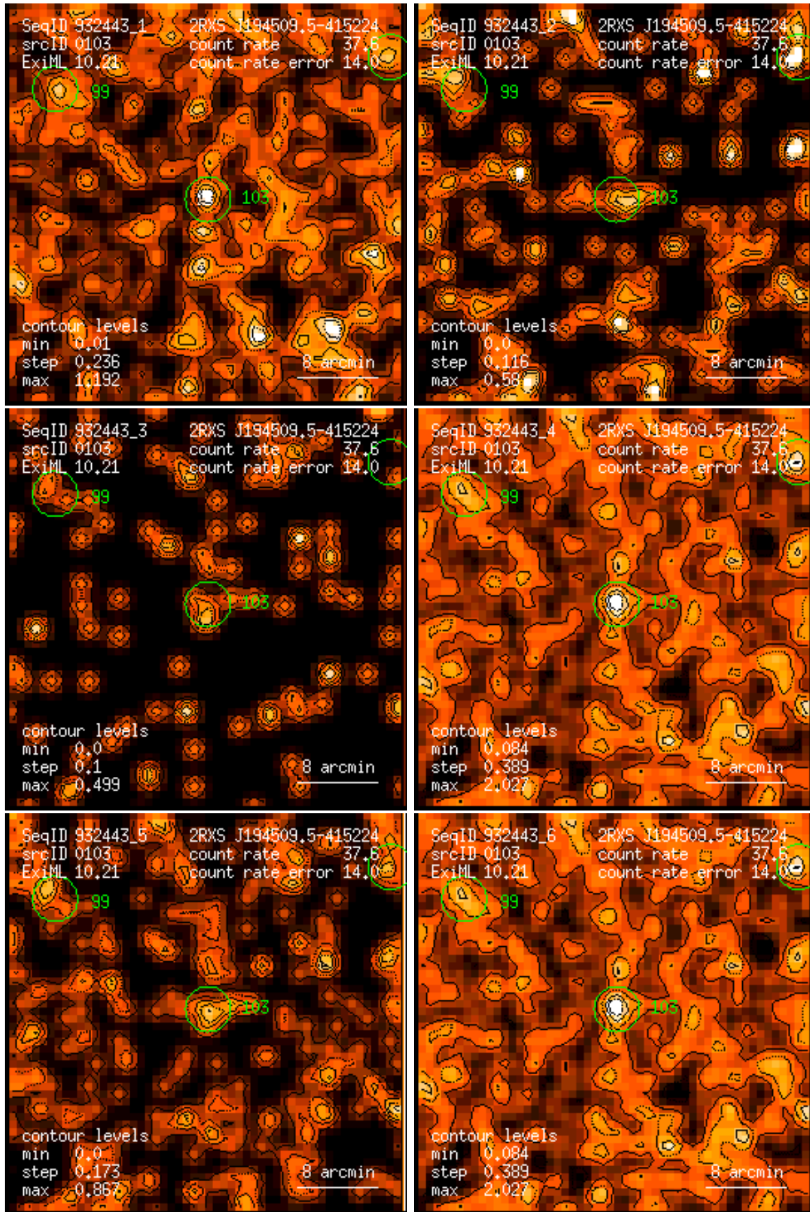
Figure 103: RASS 932443: detection 0103: band rate images, Gaussian filter: (1) PSPC channels 11 – 41, (2) 52 – 90, (3) 91 – 201, (4) 11 – 235, (5) 52 – 201, (6) 11 – 201. Broad band rates in counts/ks. Band rate contour levels in counts/ks/arcmin 2 .
