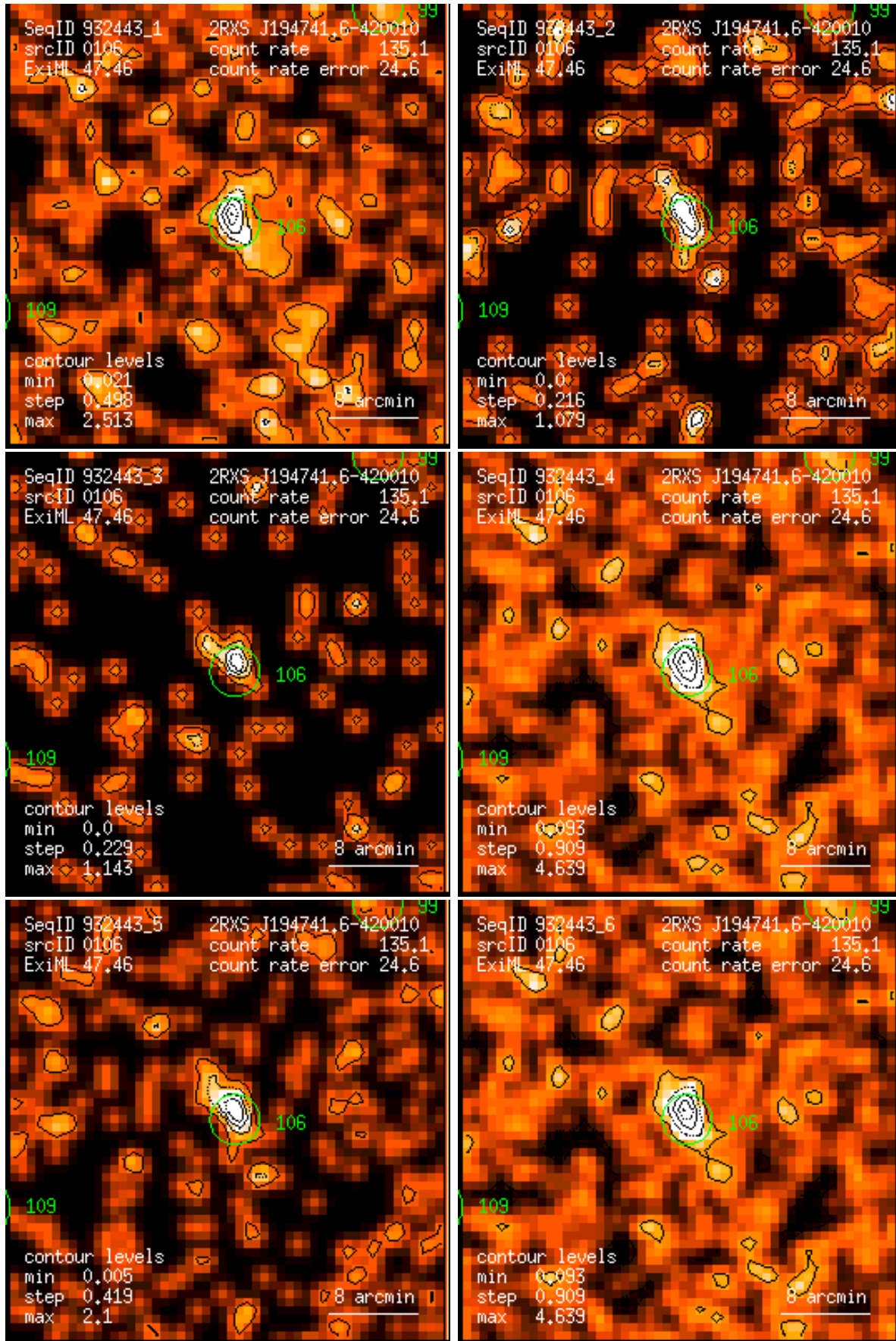
Figure 106: RASS 932443: detection 0106: band rate images, Gaussian filter: (1) PSPC channels 11 – 41, (2) 52 – 90, (3) 91 – 201, (4) 11 – 235, (5) 52 – 201, (6) 11 – 201. Broad band rates in counts/ks. Band rate contour levels in counts/ks/arcmin 2 .
