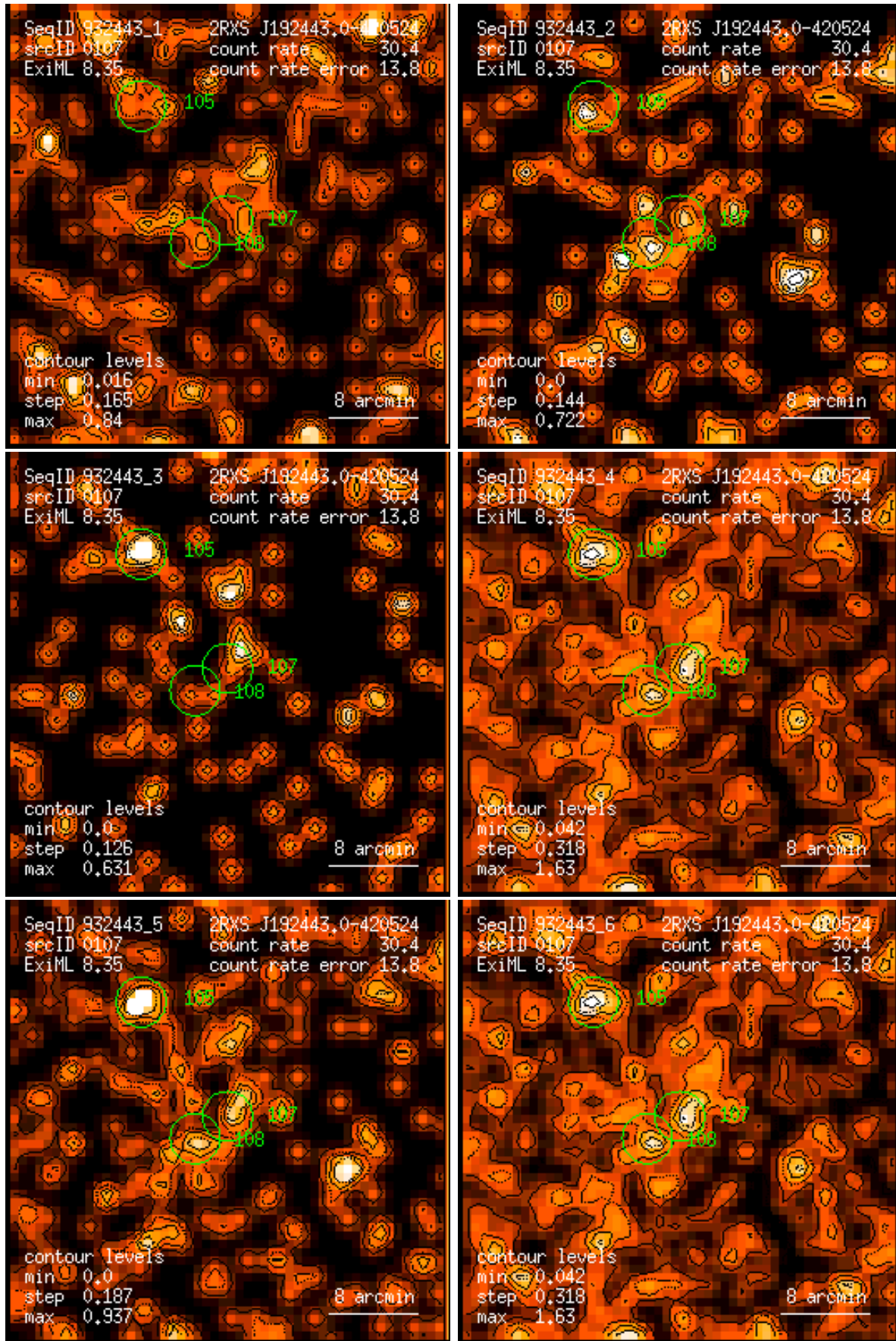
Figure 107: RASS 932443: detection 0107: band rate images, Gaussian filter: (1) PSPC channels 11 – 41, (2) 52 – 90, (3) 91 – 201, (4) 11 – 235, (5) 52 – 201, (6) 11 – 201. Broad band rates in counts/ks. Band rate contour levels in counts/ks/arcmin 2 .
