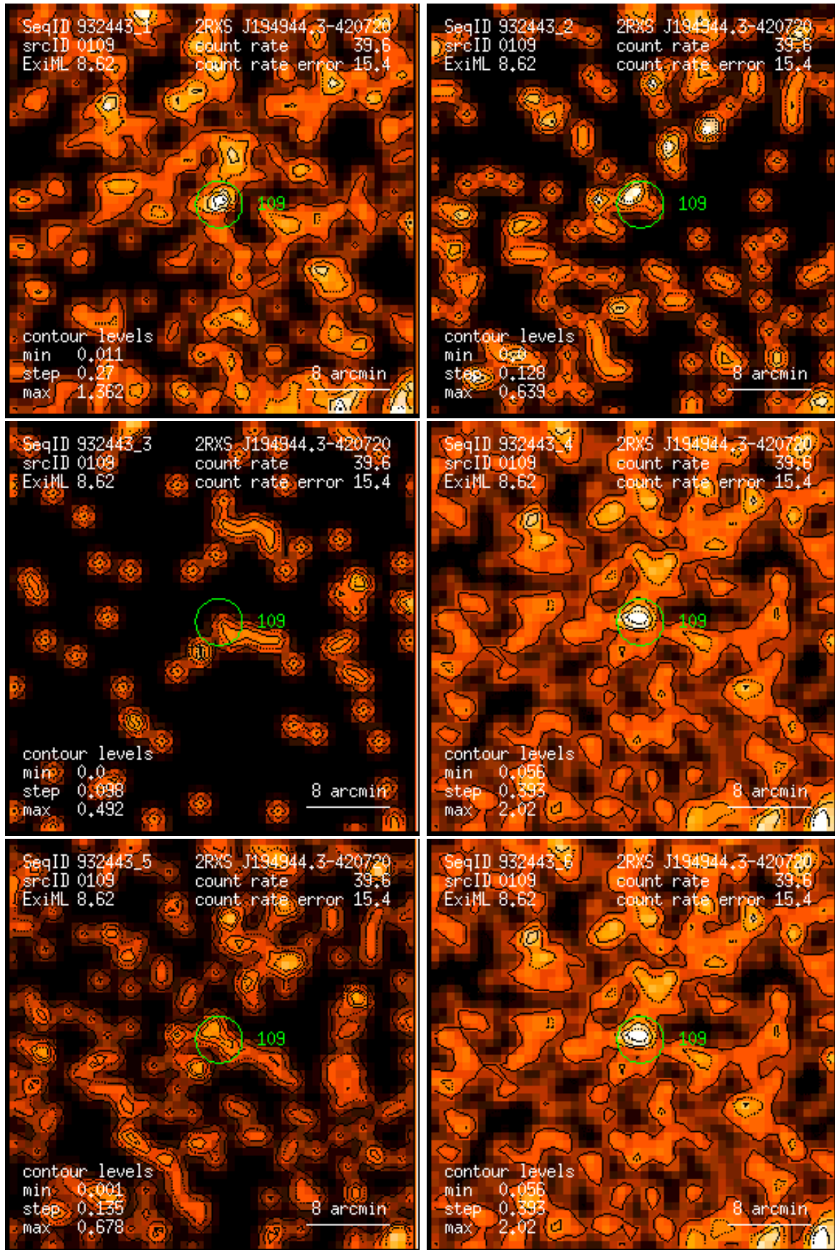
Figure 109: RASS 932443: detection 0109: band rate images, Gaussian filter: (1) PSPC channels 11 – 41, (2) 52 – 90, (3) 91 – 201, (4) 11 – 235, (5) 52 – 201, (6) 11 – 201. Broad band rates in counts/ks. Band rate contour levels in counts/ks/arcmin 2 .
