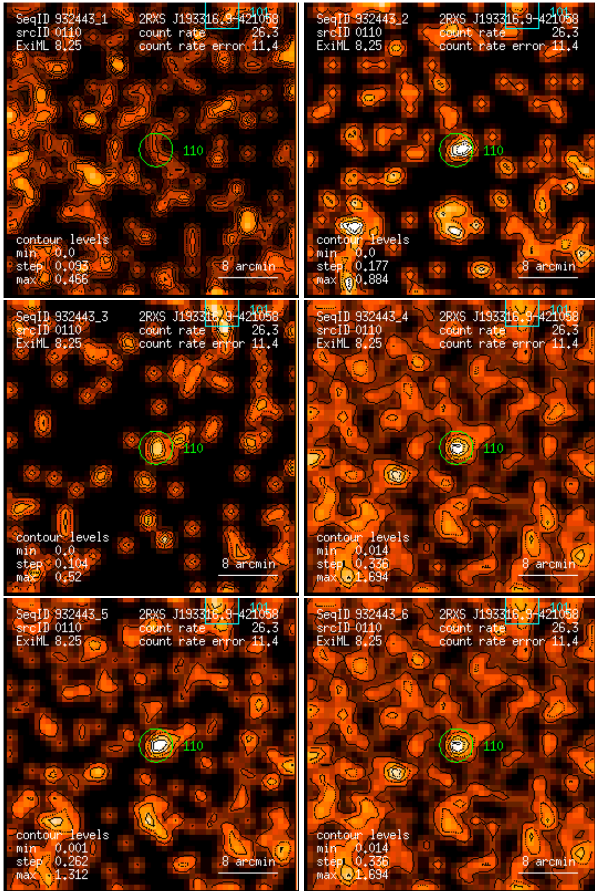
Figure 110: RASS 932443: detection 0110: band rate images, Gaussian filter: (1) PSPC channels 11 – 41, (2) 52 – 90, (3) 91 – 201, (4) 11 – 235, (5) 52 – 201, (6) 11 – 201. Broad band rates in counts/ks. Band rate contour levels in counts/ks/arcmin 2 .
