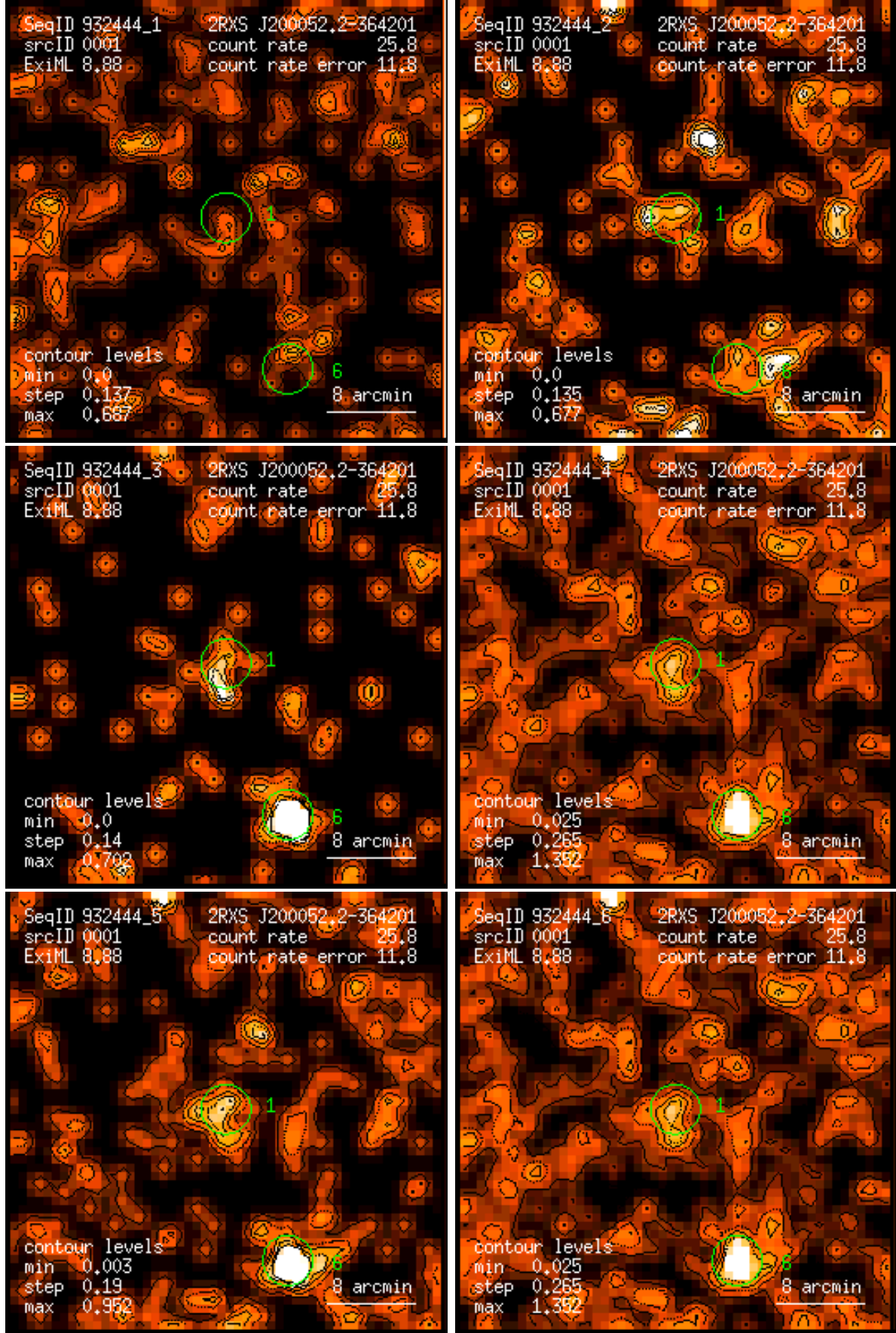
Figure 1: RASS 932444: detection 0001: band rate images, Gaussian filter: (1) PSPC channels 11 – 41, (2) 52 – 90, (3) 91 – 201, (4) 11 – 235, (5) 52 – 201, (6) 11 – 201. Broad band rates in counts/ks. Band rate contour levels in counts/ks/arcmin 2 .
