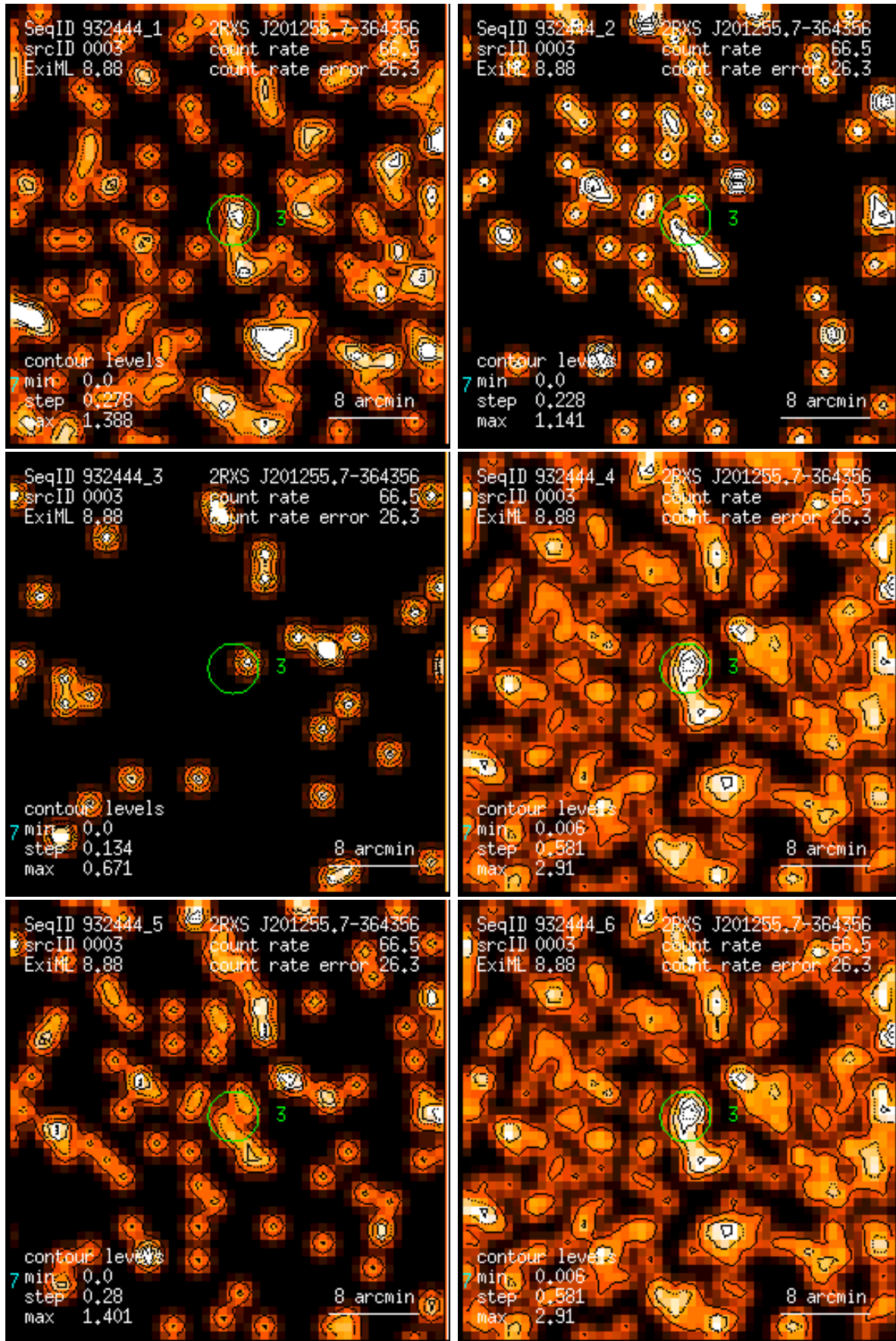
Figure 3: RASS 932444: detection 0003: band rate images, Gaussian filter: (1) PSPC channels 11 – 41, (2) 52 – 90, (3) 91 – 201, (4) 11 – 235, (5) 52 – 201, (6) 11 – 201. Broad band rates in counts/ks. Band rate contour levels in counts/ks/arcmin 2 .
