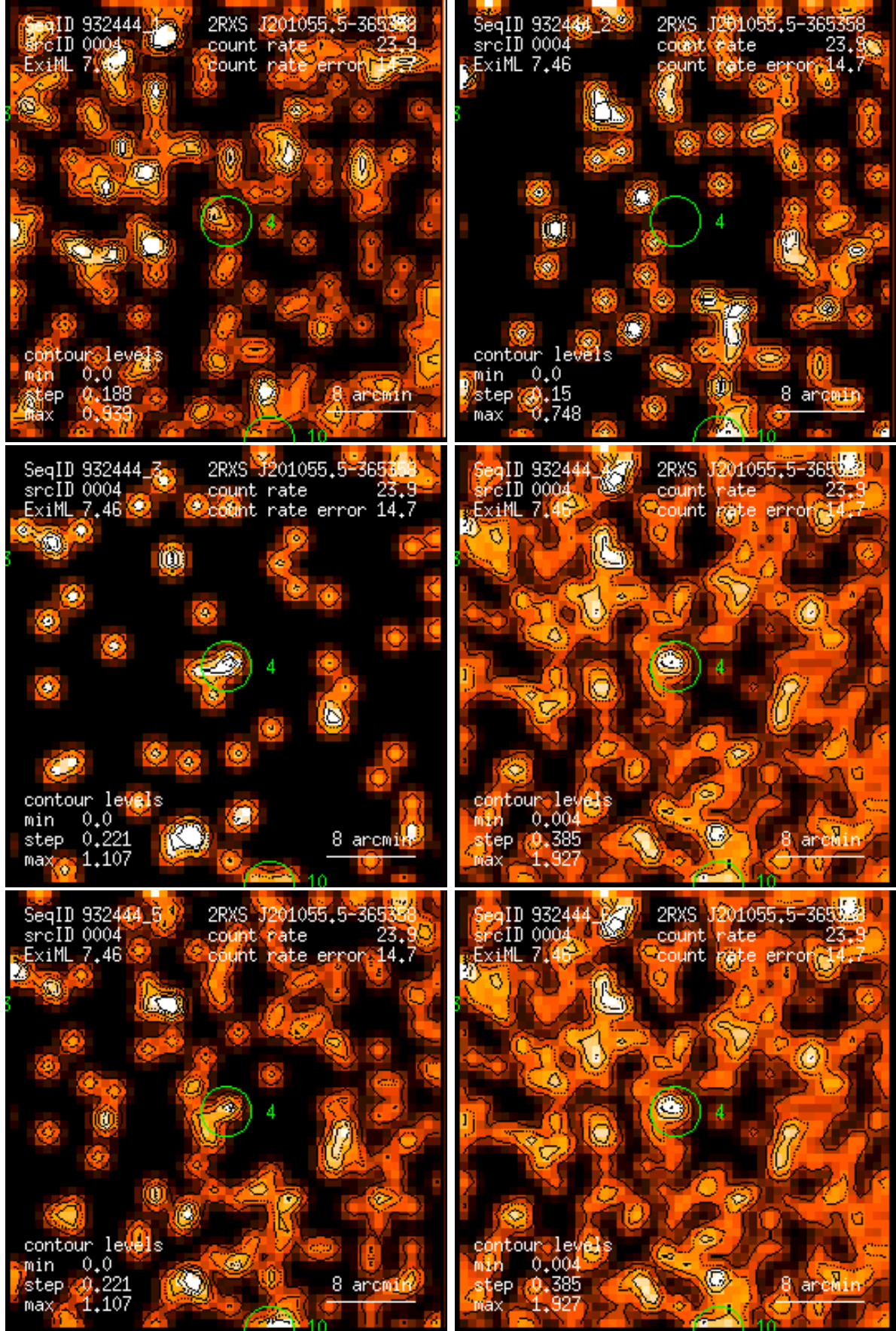
Figure 4: RASS 932444: detection 0004: band rate images, Gaussian filter: (1) PSPC channels 11 – 41, (2) 52 – 90, (3) 91 – 201, (4) 11 – 235, (5) 52 – 201, (6) 11 – 201. Broad band rates in counts/ks. Band rate contour levels in counts/ks/arcmin 2 .
