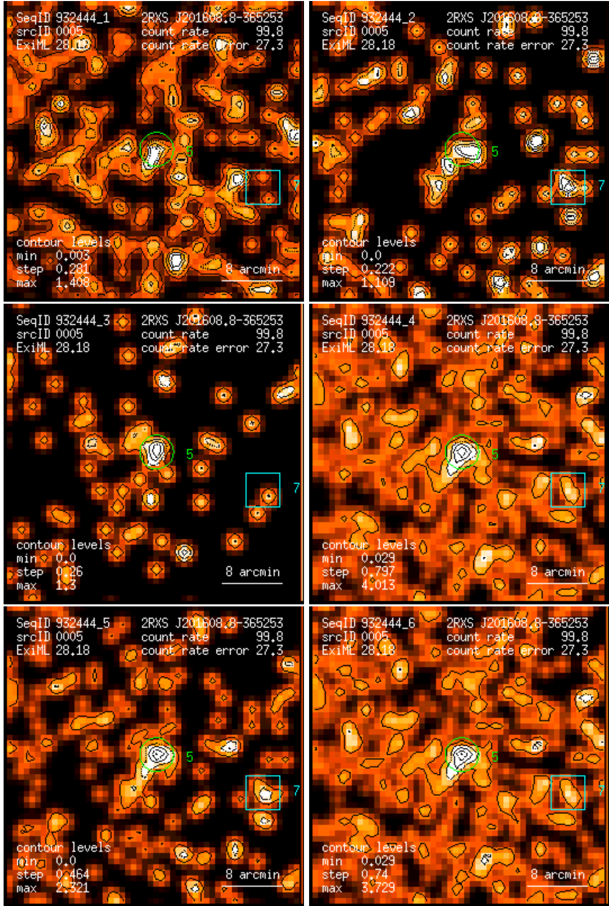
Figure 5: RASS 932444: detection 0005: band rate images, Gaussian filter: (1) PSPC channels 11 – 41, (2) 52 – 90, (3) 91 – 201, (4) 11 – 235, (5) 52 – 201, (6) 11 – 201. Broad band rates in counts/ks. Band rate contour levels in counts/ks/arcmin 2 .
