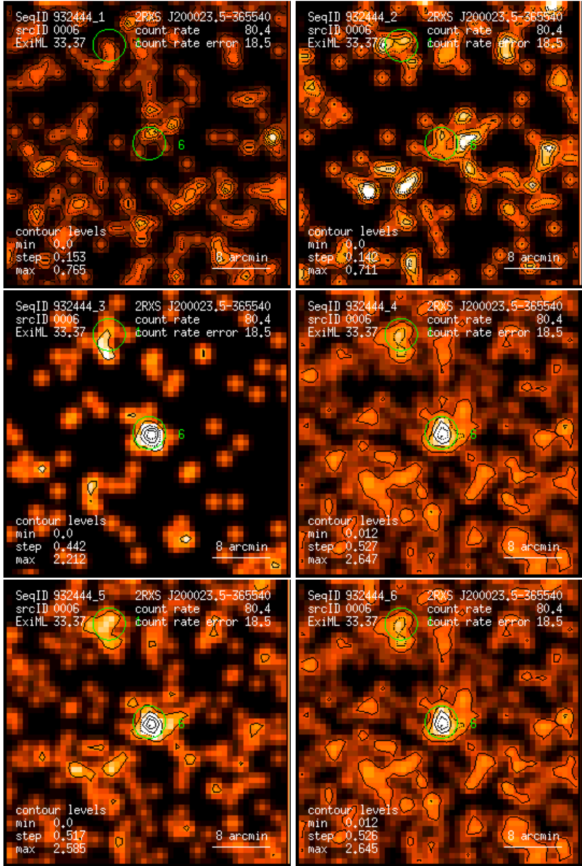
Figure 6: RASS 932444: detection 0006: band rate images, Gaussian filter: (1) PSPC channels 11 – 41, (2) 52 – 90, (3) 91 – 201, (4) 11 – 235, (5) 52 – 201, (6) 11 – 201. Broad band rates in counts/ks. Band rate contour levels in counts/ks/arcmin 2 .
