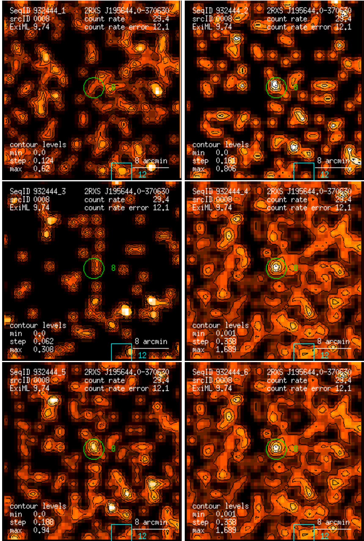
Figure 8: RASS 932444: detection 0008: band rate images, Gaussian filter: (1) PSPC channels 11 – 41, (2) 52 – 90, (3) 91 – 201, (4) 11 – 235, (5) 52 – 201, (6) 11 – 201. Broad band rates in counts/ks. Band rate contour levels in counts/ks/arcmin 2 .
