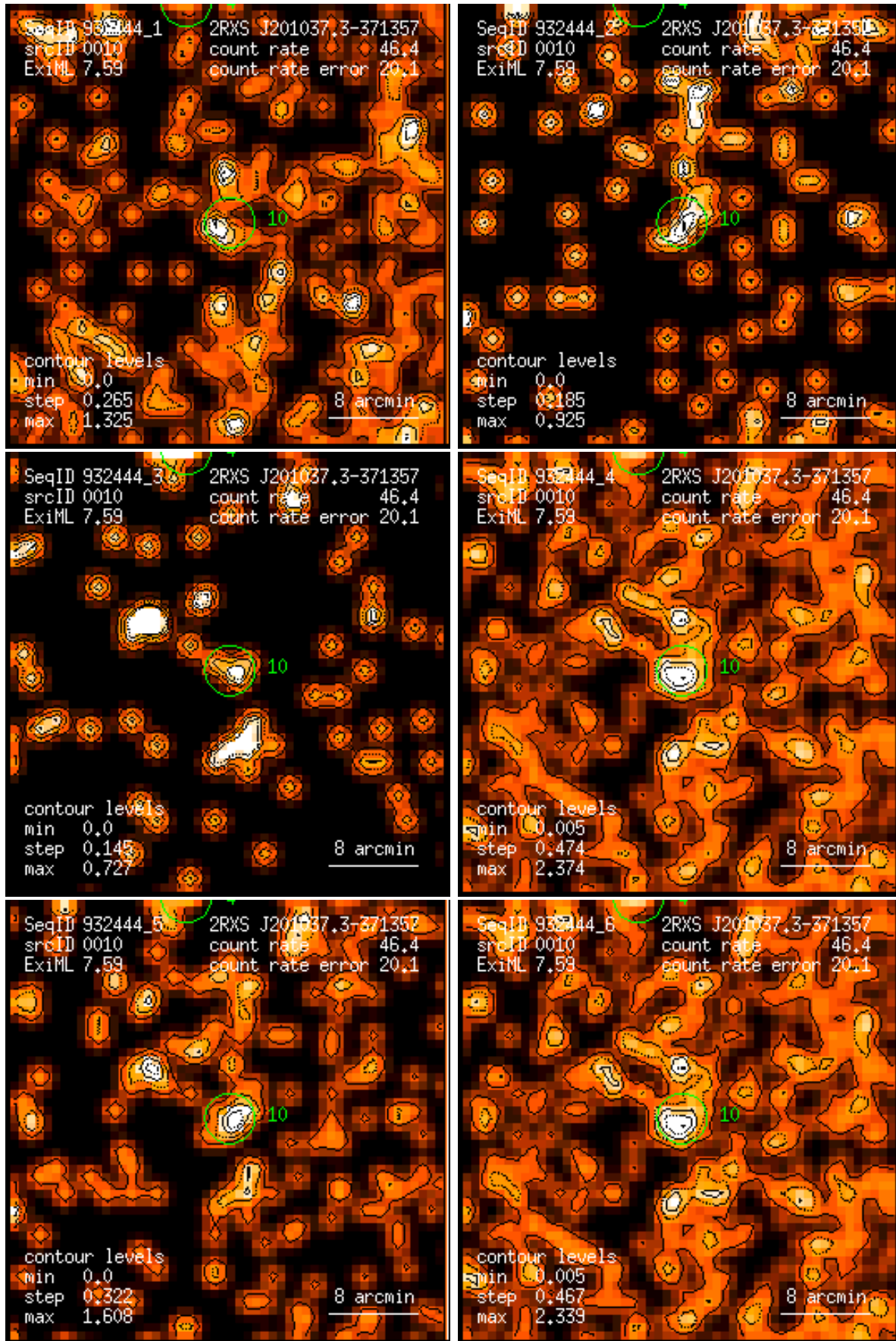
Figure 10: RASS 932444: detection 0010: band rate images, Gaussian filter: (1) PSPC channels 11 – 41, (2) 52 – 90, (3) 91 – 201, (4) 11 – 235, (5) 52 – 201, (6) 11 – 201. Broad band rates in counts/ks. Band rate contour levels in counts/ks/arcmin 2 .
