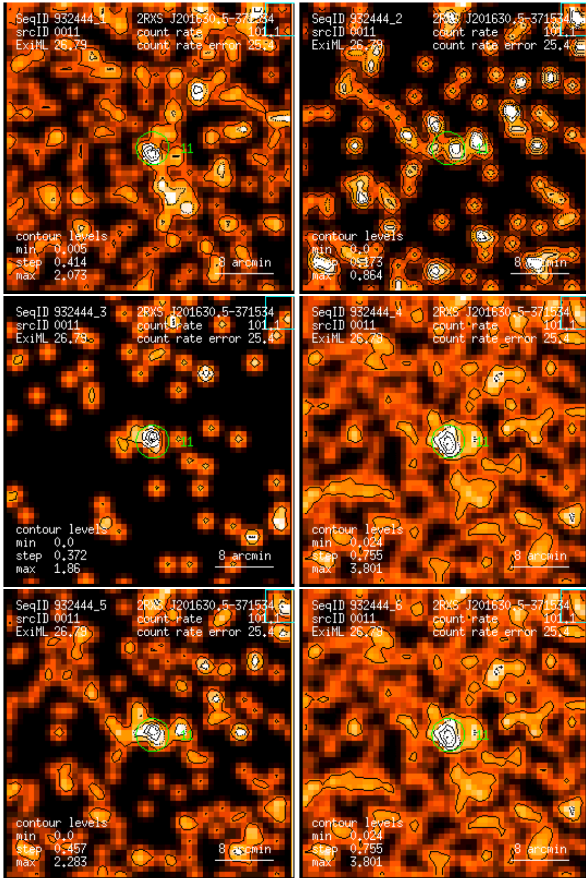
Figure 11: RASS 932444: detection 0011: band rate images, Gaussian filter: (1) PSPC channels 11 – 41, (2) 52 – 90, (3) 91 – 201, (4) 11 – 235, (5) 52 – 201, (6) 11 – 201. Broad band rates in counts/ks. Band rate contour levels in counts/ks/arcmin 2 .
