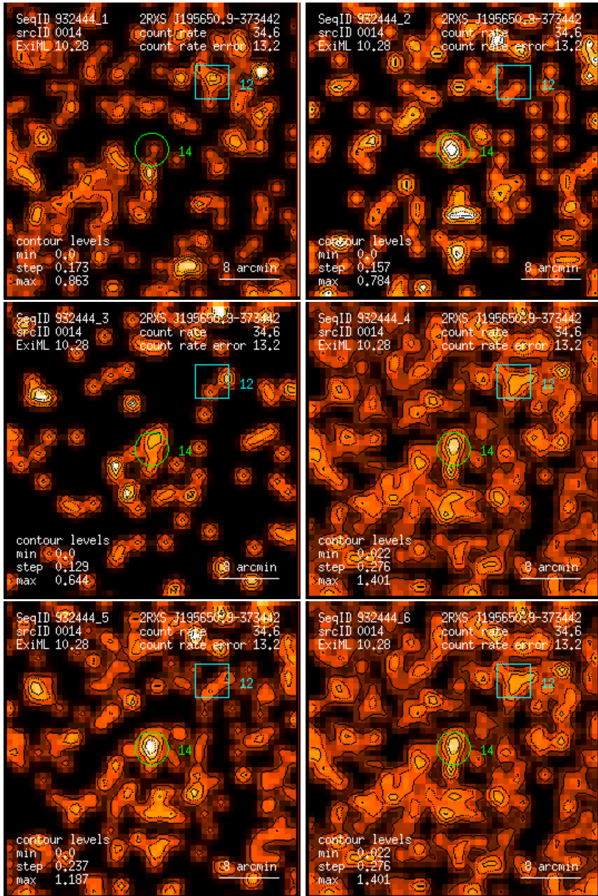
Figure 14: RASS 932444: detection 0014: band rate images, Gaussian filter: (1) PSPC channels 11 – 41, (2) 52 – 90, (3) 91 – 201, (4) 11 – 235, (5) 52 – 201, (6) 11 – 201. Broad band rates in counts/ks. Band rate contour levels in counts/ks/arcmin 2 .
