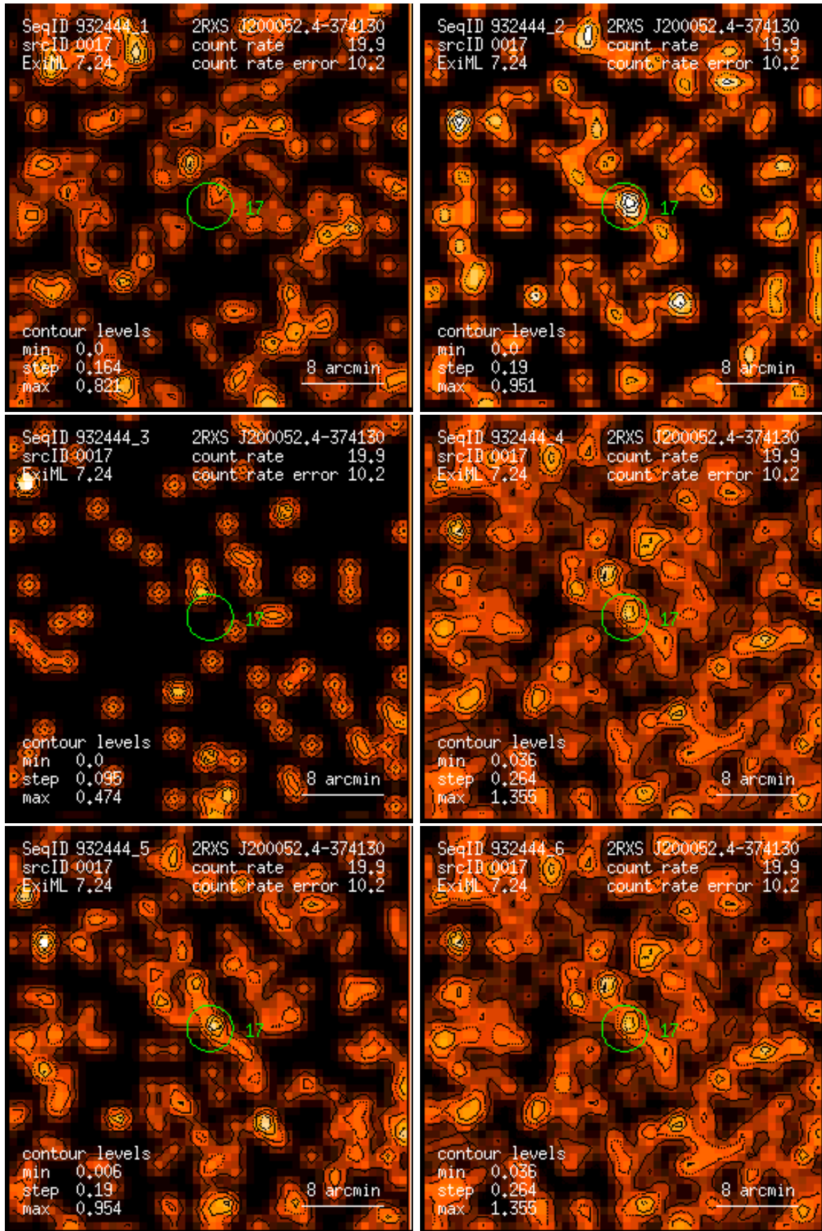
Figure 17: RASS 932444: detection 0017: band rate images, Gaussian filter: (1) PSPC channels 11 – 41, (2) 52 – 90, (3) 91 – 201, (4) 11 – 235, (5) 52 – 201, (6) 11 – 201. Broad band rates in counts/ks. Band rate contour levels in counts/ks/arcmin 2 .
