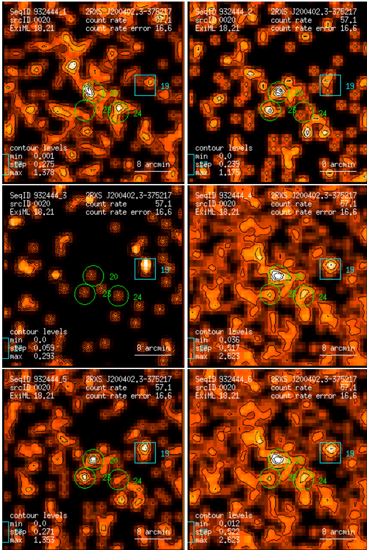
Figure 20: RASS 932444: detection 0020: band rate images, Gaussian filter: (1) PSPC channels 11 – 41, (2) 52 – 90, (3) 91 – 201, (4) 11 – 235, (5) 52 – 201, (6) 11 – 201. Broad band rates in counts/ks. Band rate contour levels in counts/ks/arcmin 2 .
