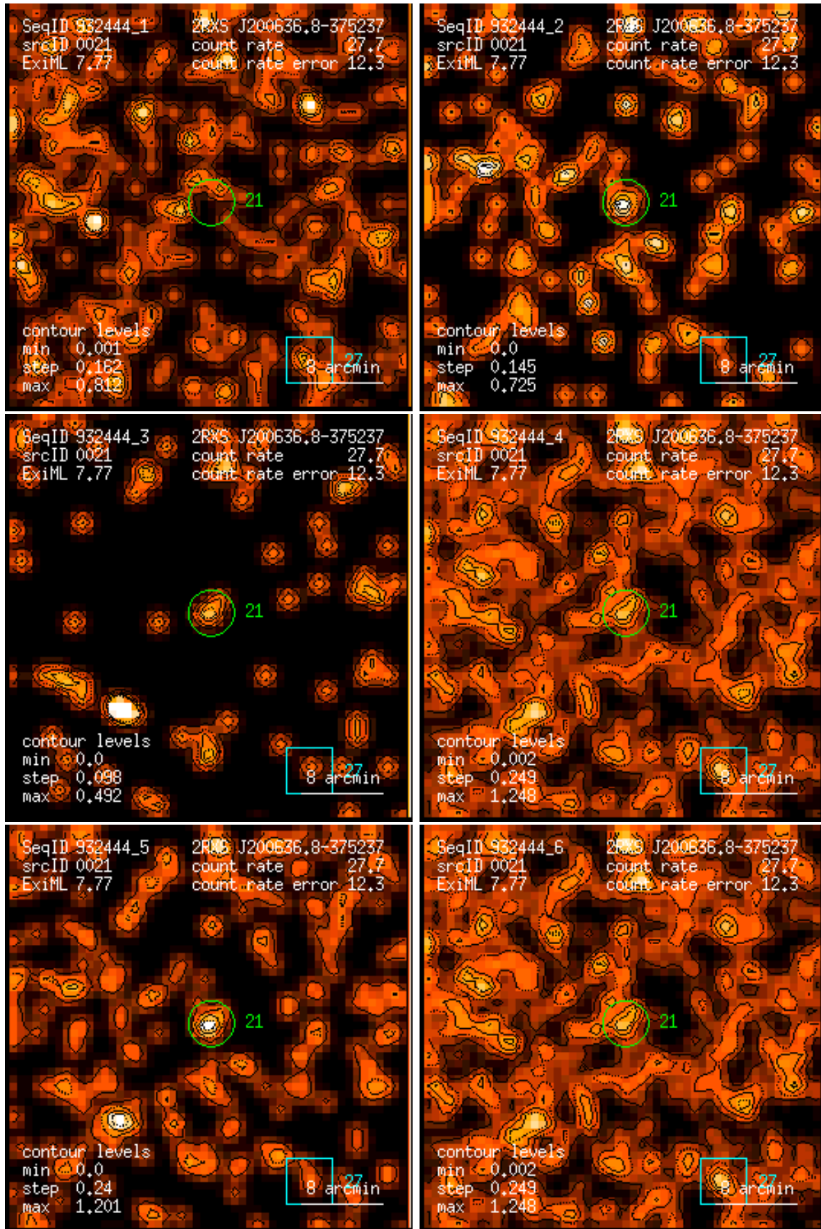
Figure 21: RASS 932444: detection 0021: band rate images, Gaussian filter: (1) PSPC channels 11 – 41, (2) 52 – 90, (3) 91 – 201, (4) 11 – 235, (5) 52 – 201, (6) 11 – 201. Broad band rates in counts/ks. Band rate contour levels in counts/ks/arcmin 2 .
