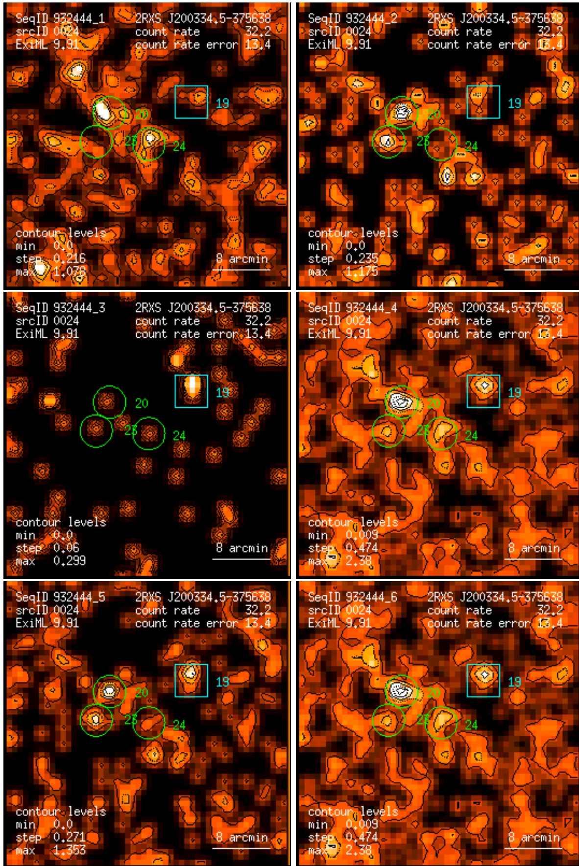
Figure 24: RASS 932444: detection 0024: band rate images, Gaussian filter: (1) PSPC channels 11 – 41, (2) 52 – 90, (3) 91 – 201, (4) 11 – 235, (5) 52 – 201, (6) 11 – 201. Broad band rates in counts/ks. Band rate contour levels in counts/ks/arcmin 2 .
