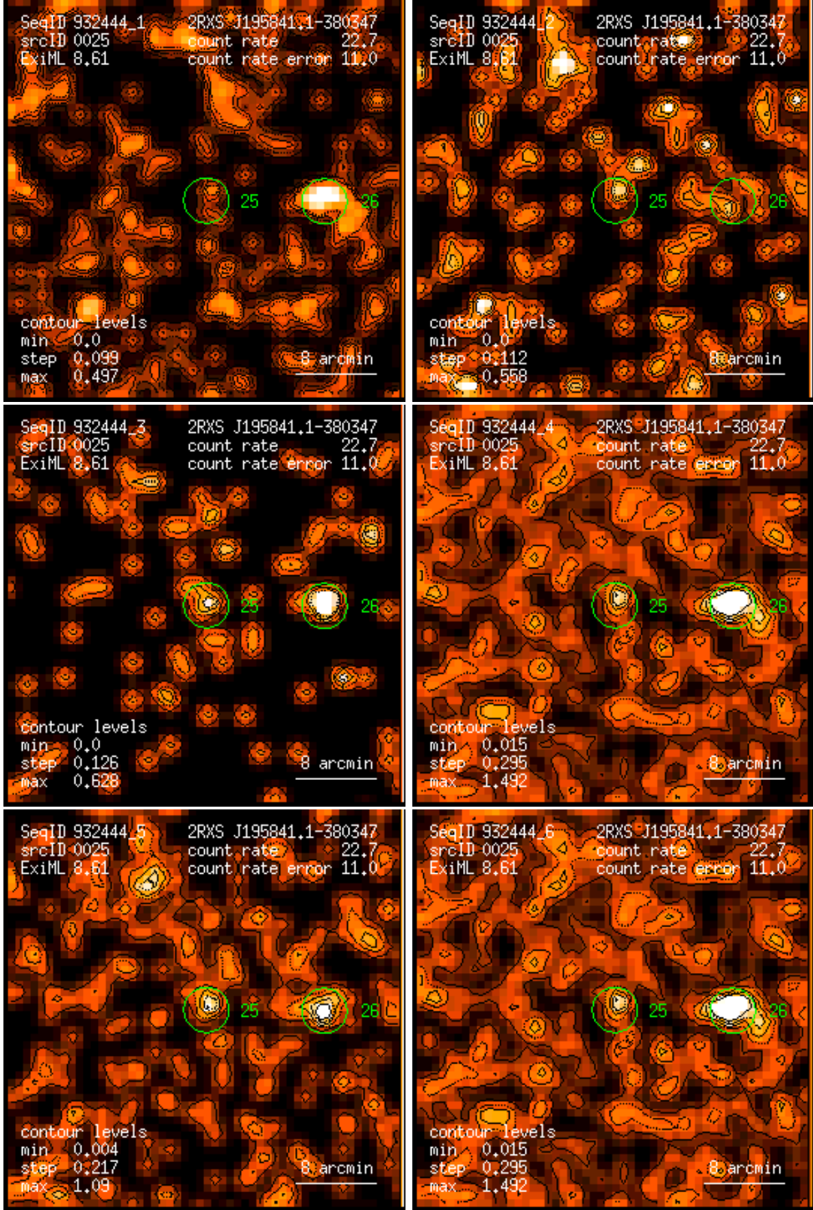
Figure 25: RASS 932444: detection 0025: band rate images, Gaussian filter: (1) PSPC channels 11 – 41, (2) 52 – 90, (3) 91 – 201, (4) 11 – 235, (5) 52 – 201, (6) 11 – 201. Broad band rates in counts/ks. Band rate contour levels in counts/ks/arcmin 2 .
