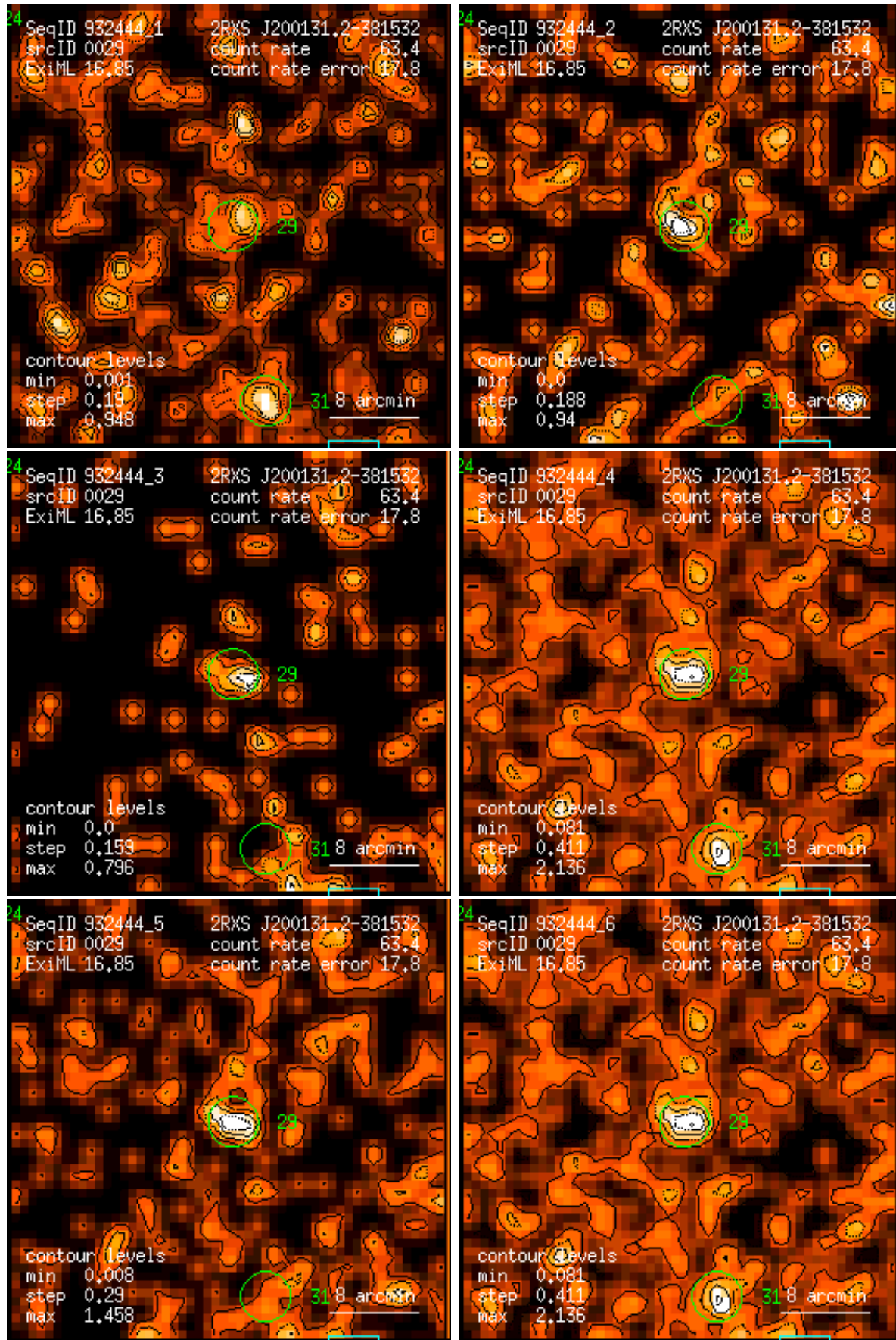
Figure 29: RASS 932444: detection 0029: band rate images, Gaussian filter: (1) PSPC channels 11 – 41, (2) 52 – 90, (3) 91 – 201, (4) 11 – 235, (5) 52 – 201, (6) 11 – 201. Broad band rates in counts/ks. Band rate contour levels in counts/ks/arcmin 2 .
