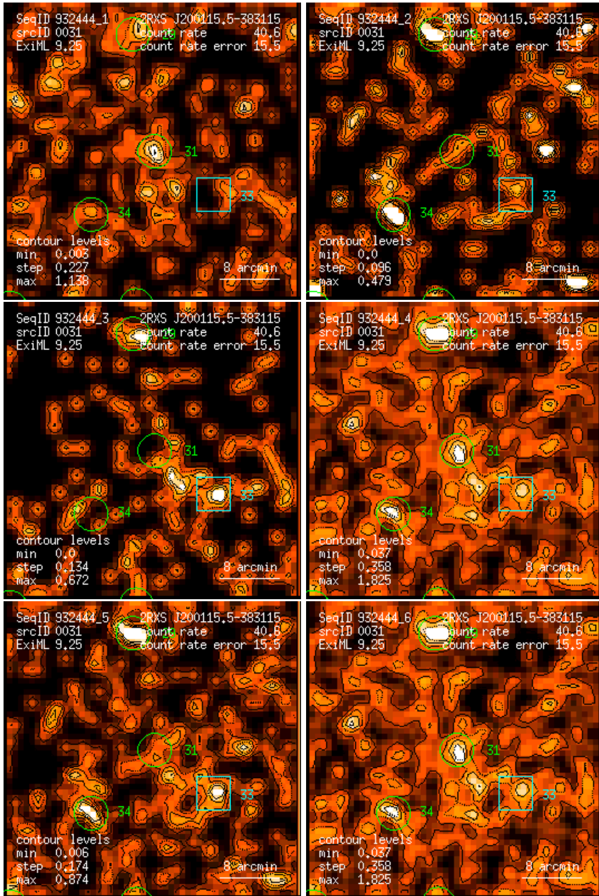
Figure 31: RASS 932444: detection 0031: band rate images, Gaussian filter: (1) PSPC channels 11 – 41, (2) 52 – 90, (3) 91 – 201, (4) 11 – 235, (5) 52 – 201, (6) 11 – 201. Broad band rates in counts/ks. Band rate contour levels in counts/ks/arcmin 2 .
