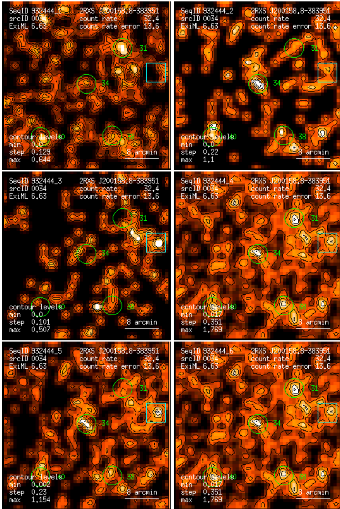
Figure 34: RASS 932444: detection 0034: band rate images, Gaussian filter: (1) PSPC channels 11 – 41, (2) 52 – 90, (3) 91 – 201, (4) 11 – 235, (5) 52 – 201, (6) 11 – 201. Broad band rates in counts/ks. Band rate contour levels in counts/ks/arcmin 2 .
