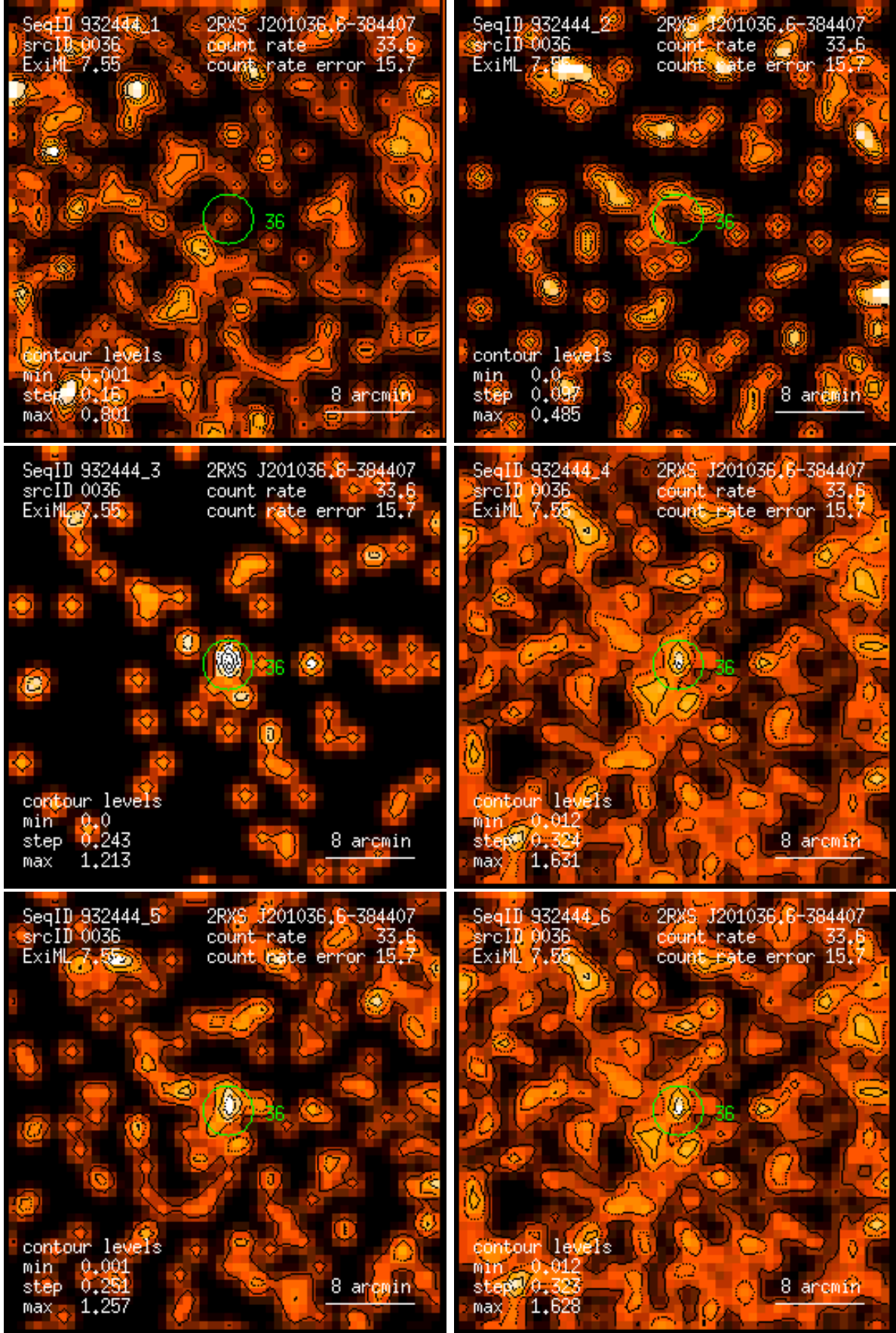
Figure 36: RASS 932444: detection 0036: band rate images, Gaussian filter: (1) PSPC channels 11 – 41, (2) 52 – 90, (3) 91 – 201, (4) 11 – 235, (5) 52 – 201, (6) 11 – 201. Broad band rates in counts/ks. Band rate contour levels in counts/ks/arcmin 2 .
