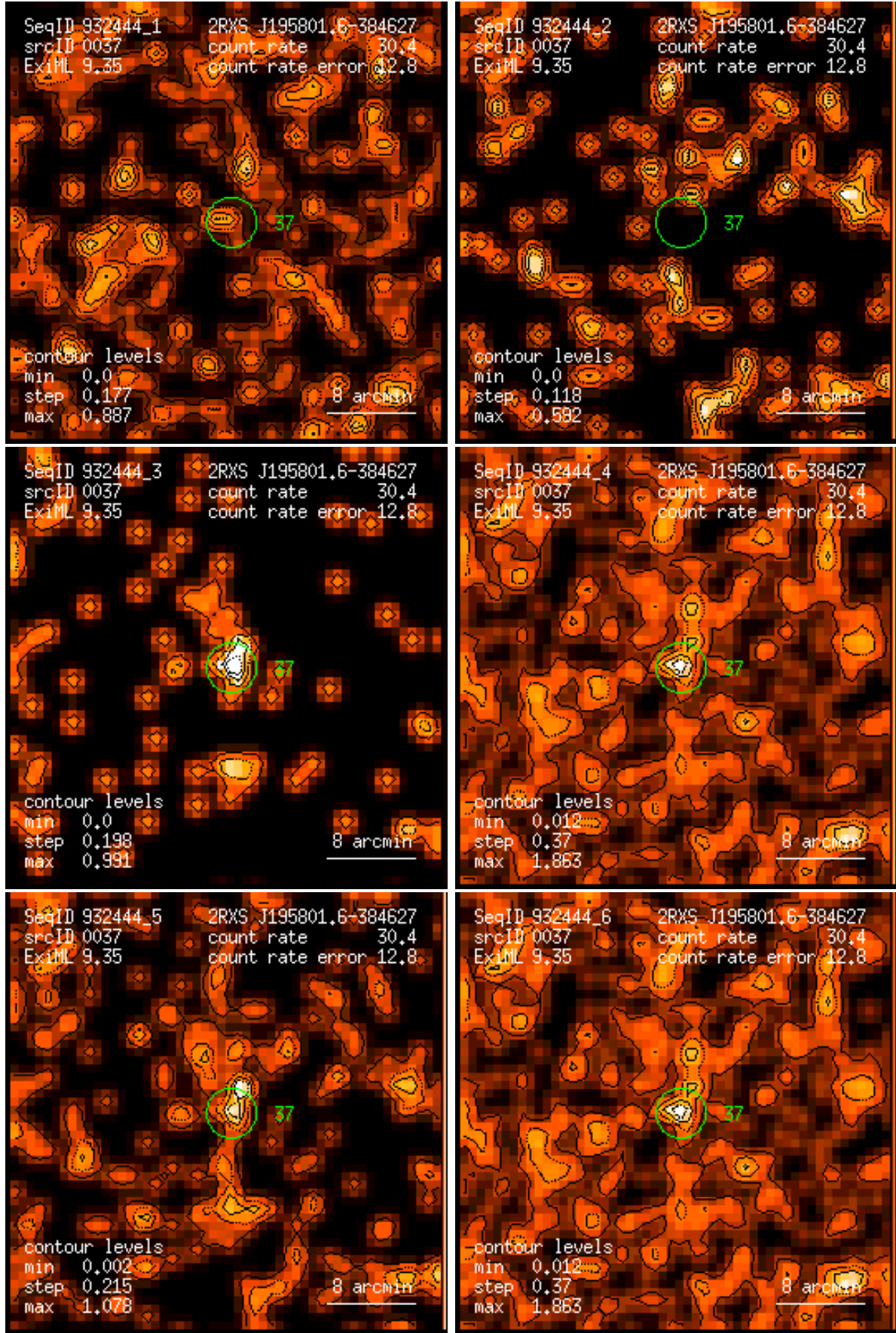
Figure 37: RASS 932444: detection 0037: band rate images, Gaussian filter: (1) PSPC channels 11 – 41, (2) 52 – 90, (3) 91 – 201, (4) 11 – 235, (5) 52 – 201, (6) 11 – 201. Broad band rates in counts/ks. Band rate contour levels in counts/ks/arcmin 2 .
