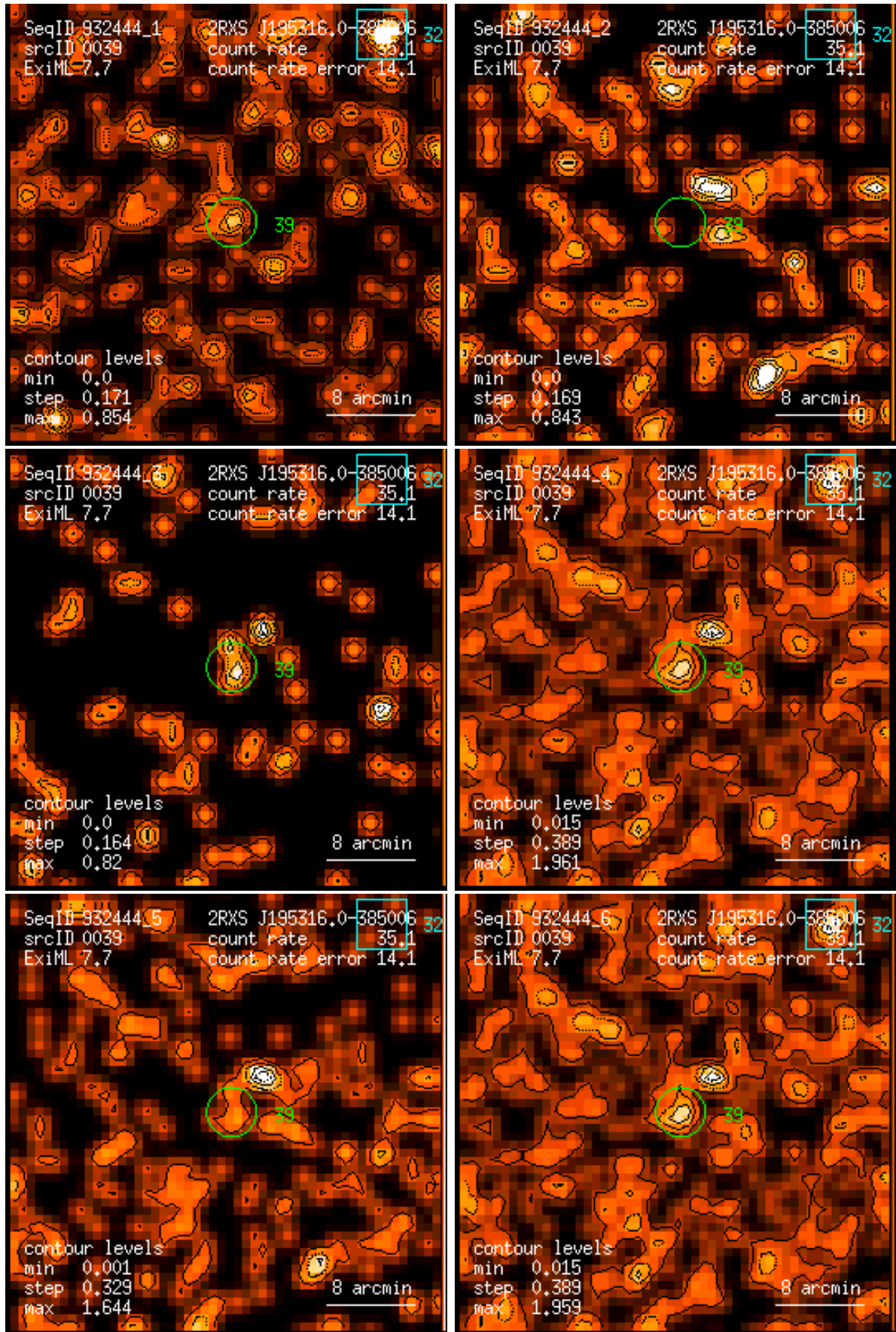
Figure 39: RASS 932444: detection 0039: band rate images, Gaussian filter: (1) PSPC channels 11 – 41, (2) 52 – 90, (3) 91 – 201, (4) 11 – 235, (5) 52 – 201, (6) 11 – 201. Broad band rates in counts/ks. Band rate contour levels in counts/ks/arcmin 2 .
