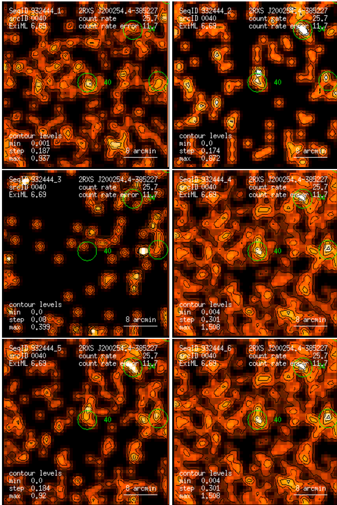
Figure 40: RASS 932444: detection 0040: band rate images, Gaussian filter: (1) PSPC channels 11 – 41, (2) 52 – 90, (3) 91 – 201, (4) 11 – 235, (5) 52 – 201, (6) 11 – 201. Broad band rates in counts/ks. Band rate contour levels in counts/ks/arcmin 2 .
