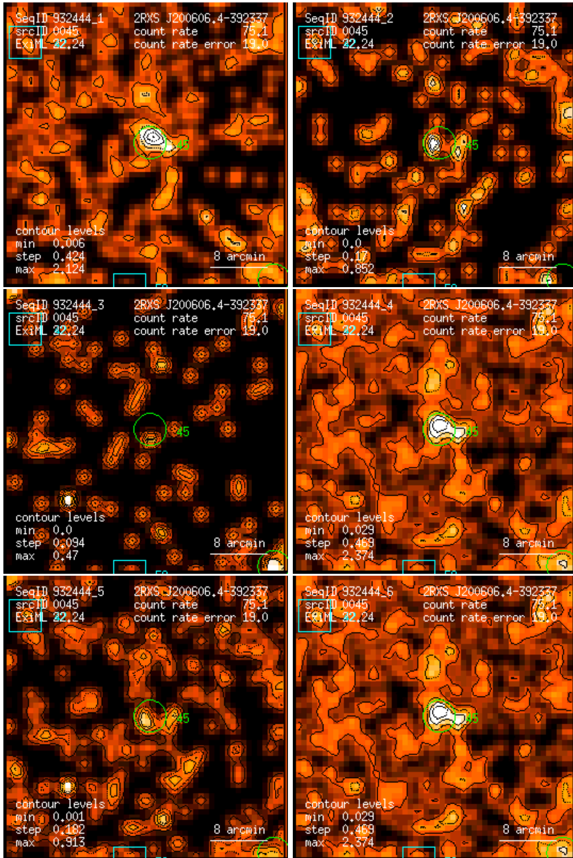
Figure 45: RASS 932444: detection 0045: band rate images, Gaussian filter: (1) PSPC channels 11 – 41, (2) 52 – 90, (3) 91 – 201, (4) 11 – 235, (5) 52 – 201, (6) 11 – 201. Broad band rates in counts/ks. Band rate contour levels in counts/ks/arcmin 2 .
