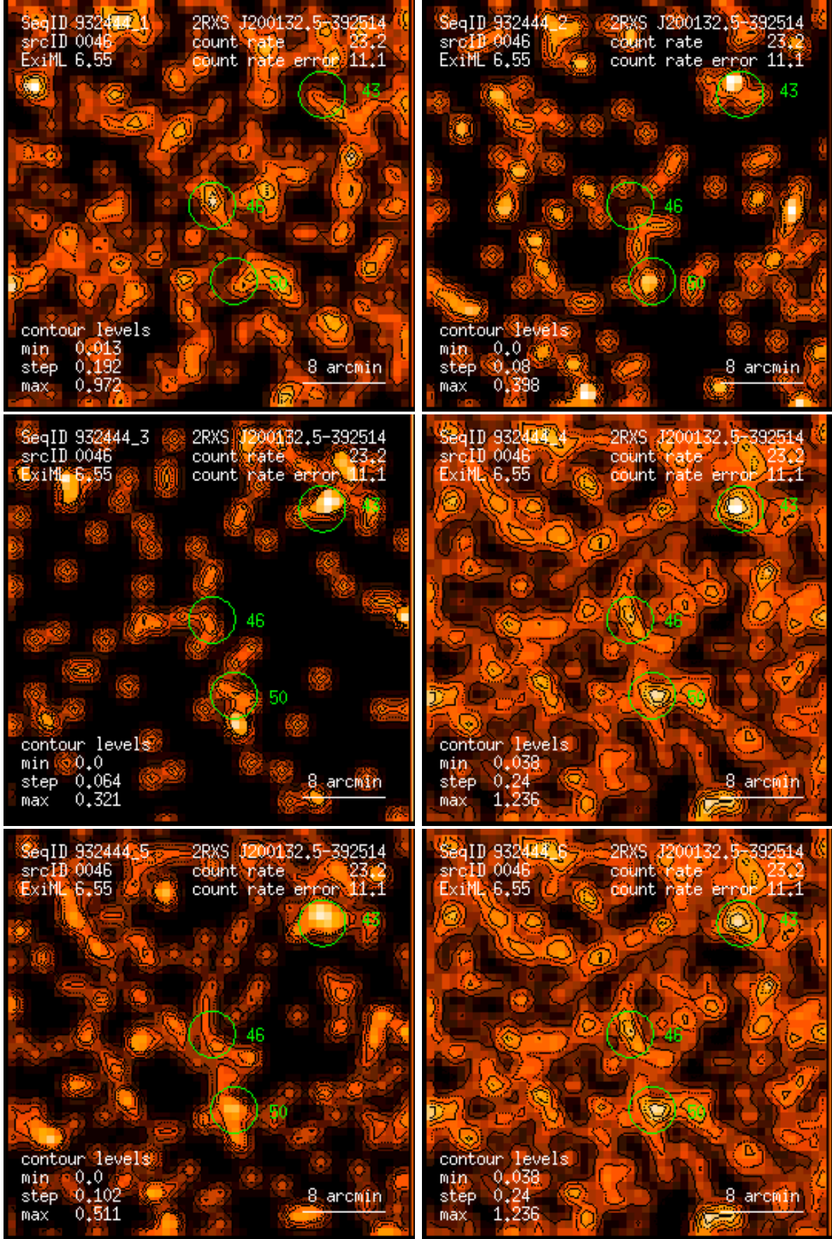
Figure 46: RASS 932444: detection 0046: band rate images, Gaussian filter: (1) PSPC channels 11 – 41, (2) 52 – 90, (3) 91 – 201, (4) 11 – 235, (5) 52 – 201, (6) 11 – 201. Broad band rates in counts/ks. Band rate contour levels in counts/ks/arcmin 2 .
