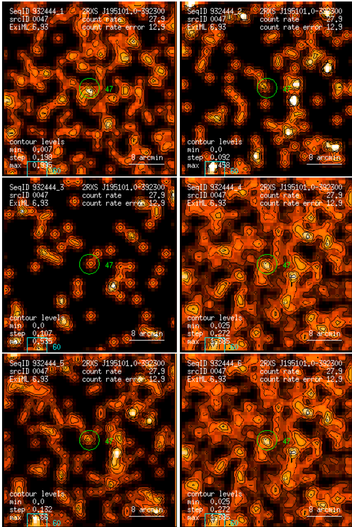
Figure 47: RASS 932444: detection 0047: band rate images, Gaussian filter: (1) PSPC channels 11 – 41, (2) 52 – 90, (3) 91 – 201, (4) 11 – 235, (5) 52 – 201, (6) 11 – 201. Broad band rates in counts/ks. Band rate contour levels in counts/ks/arcmin 2 .
