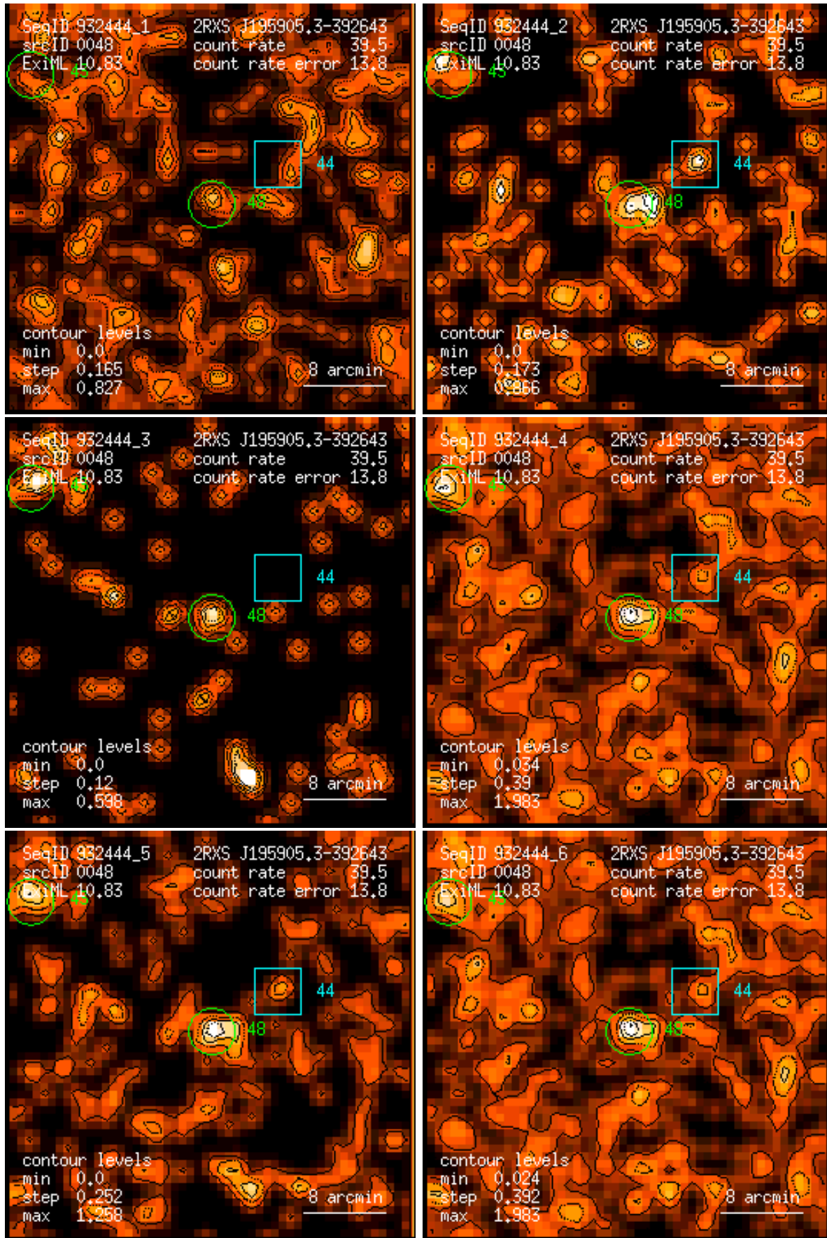
Figure 48: RASS 932444: detection 0048: band rate images, Gaussian filter: (1) PSPC channels 11 – 41, (2) 52 – 90, (3) 91 – 201, (4) 11 – 235, (5) 52 – 201, (6) 11 – 201. Broad band rates in counts/ks. Band rate contour levels in counts/ks/arcmin 2 .
