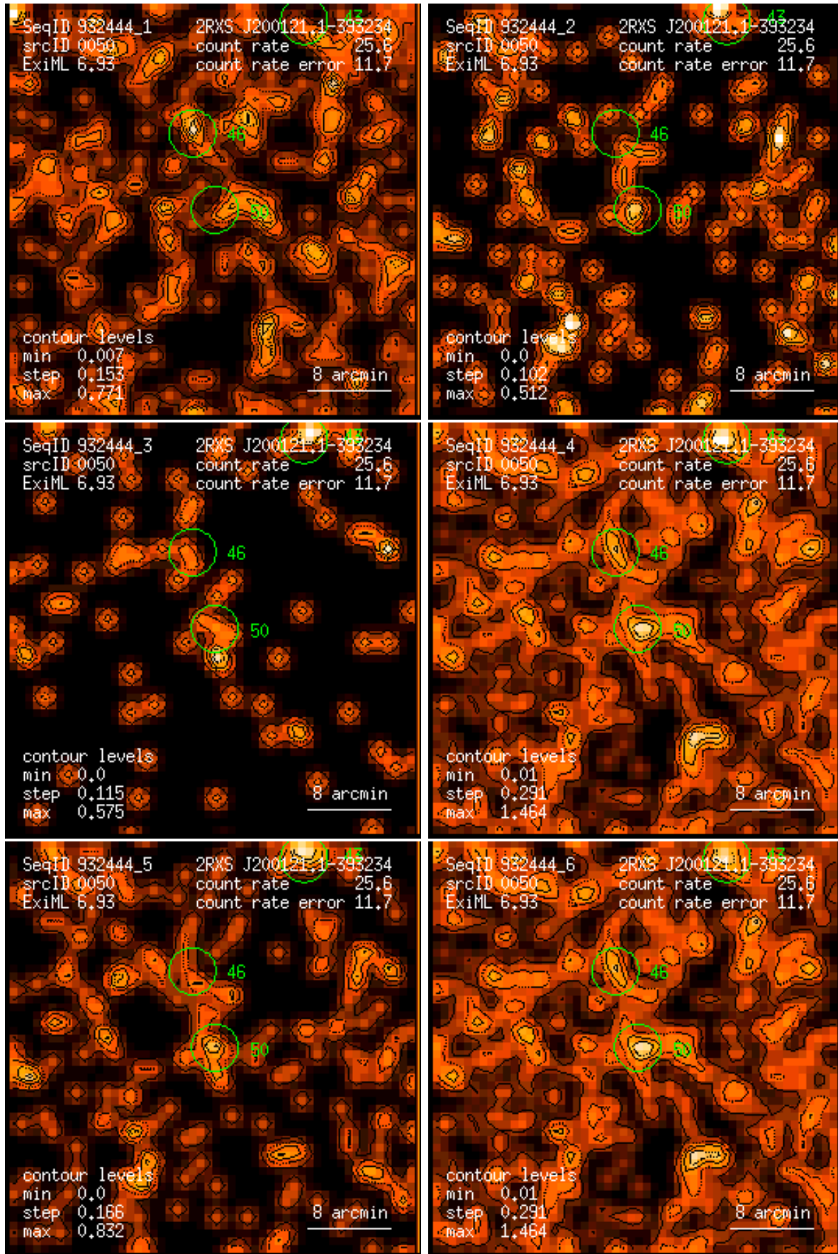
Figure 50: RASS 932444: detection 0050: band rate images, Gaussian filter: (1) PSPC channels 11 – 41, (2) 52 – 90, (3) 91 – 201, (4) 11 – 235, (5) 52 – 201, (6) 11 – 201. Broad band rates in counts/ks. Band rate contour levels in counts/ks/arcmin 2 .
